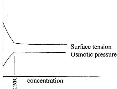
Figure 3. Representation of changes in two properties in determining the CMC of a surfactant.
