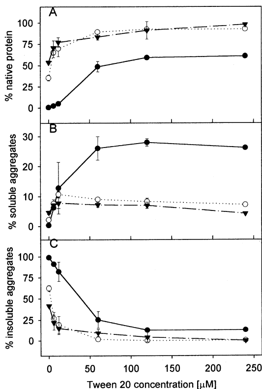
Figure 4. Recovery of native rFXIII (A) and formation of soluble (B) and insoluble aggregates (C) following 10 freeze-thaw cycles of 1 mg/ml (—●—), 5 mg/ml (····○····) and 10 mg/ml rFXIII (—▼—) as a function of Tween 20. Results are plotted as mean values \pm standard deviation for duplicate samples (reproduced from Kreilgaard et al., 1998).
