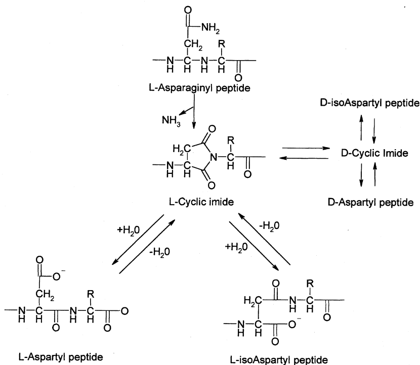
Figure 1. General mechanistic scheme for deamidation of asparagine (Asn) residues in peptide and proteins.
