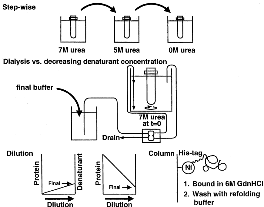
Figure 4. Diagrams of different protocols to reduce denaturant concentration.
