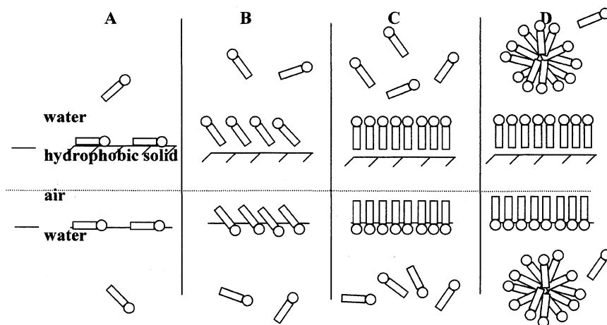
Figure 2. Simplified models of the interfacial behavior of a nonionic surfactant at several concentrations in water. Circles—polar head groups (e.g., polyoxyethlenes). Rectangles—hydrophobic tails (e.g., hydrocarbon chains). Models above the dotted line is for the hydrophobic solid (ice)/water interface and those below are for the air/water interface. (A) Surfactant concentration is well below the CMC (B) Surfactant concentration is greater than in A, but still below the CMC. (C) Surfactant concentration is at the CMC. (D) The surfactant concentration is above the CMC. (This model is adapted from Figures 4.4 and 4.8 of Porter (Porter, 1994)).
