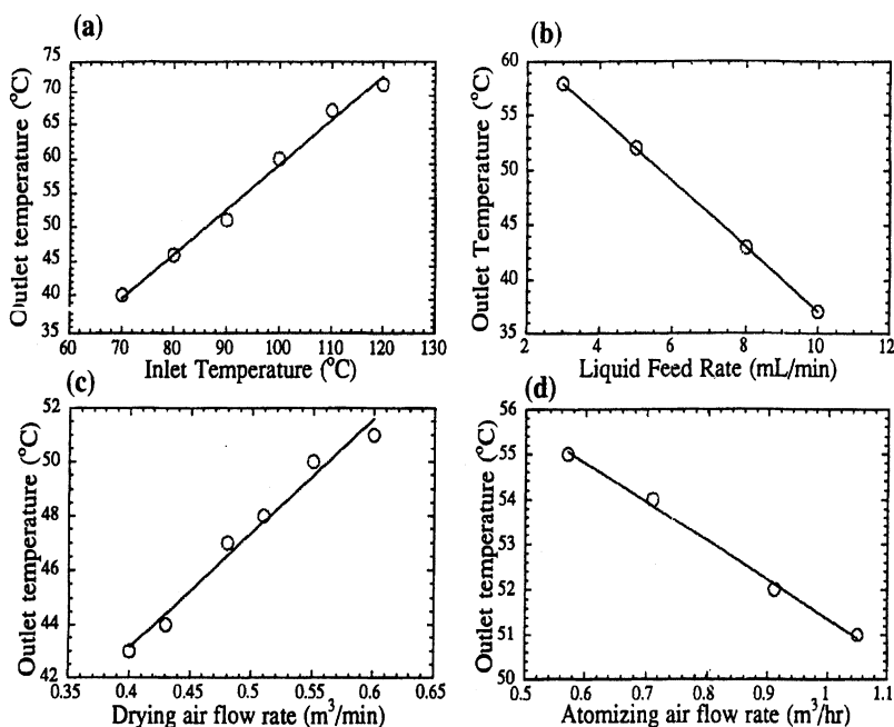
Figure 2. Measured dependencies of T_{\text{outlet}} in the Büchi laboratory spray-dryer on (a) T_{\text{inlet}} ; (b) v_{\text{lf}} ; (c) v_{\text{da}} ; (d) v_{\text{aa}} . Standard spray-drying conditions used were: T_{\text{inlet}} = 90^{\circ}\text{C} , v_{\text{lf}} = 5 \text{ mL/min} , v_{\text{da}} = 900 \text{ L/h} , v_{\text{aa}} = 600 \text{ L/min} . Figure reproduced from Maa et al. (1997), with permission.
