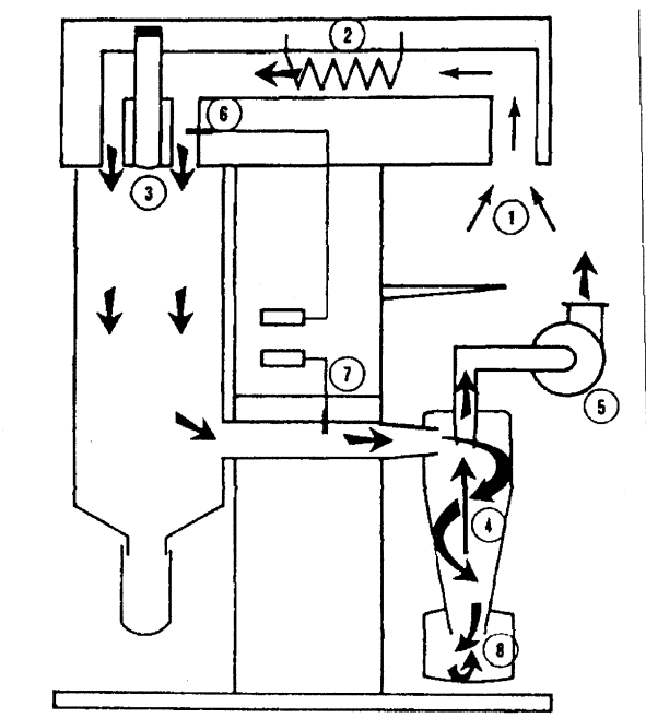
Figure 1. Schematic of Büchi laboratory spray dryer. (1) air inlet; (2) inlet-air heating element; (3) two-fluid nozzle; (4) cyclone separator; (5) ventilator fan; (6) thermocouple to measure T_{inlet} ; (7) thermocouple to measure T_{outlet} ; (8) product collector. Reproduced with permission of the manufacturer.
