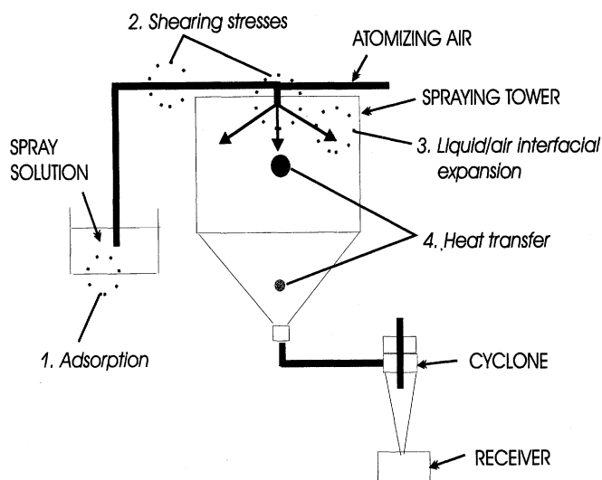
Figure 6. Schematic representation of the possible stresses experienced by a protein during spray-drying. See text for explanations. The current state of knowledge indicates that protein adsorption at the large liquid/air interface created during atomizing of the spray solution is mainly responsible for the protein aggregation/inactivation measured on spray-drying (“process instability” of the protein).
