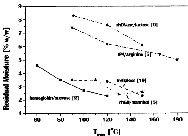
Figure 3. Relation between residual moisture and T_{inlet} for various spray-dried powders taken from the reference cited in the figure. The other independent process parameters ( v_g , v_{aa} & v_{da} ) were not in all cases the same in the various works. See text for explanations of the abbreviations used.
