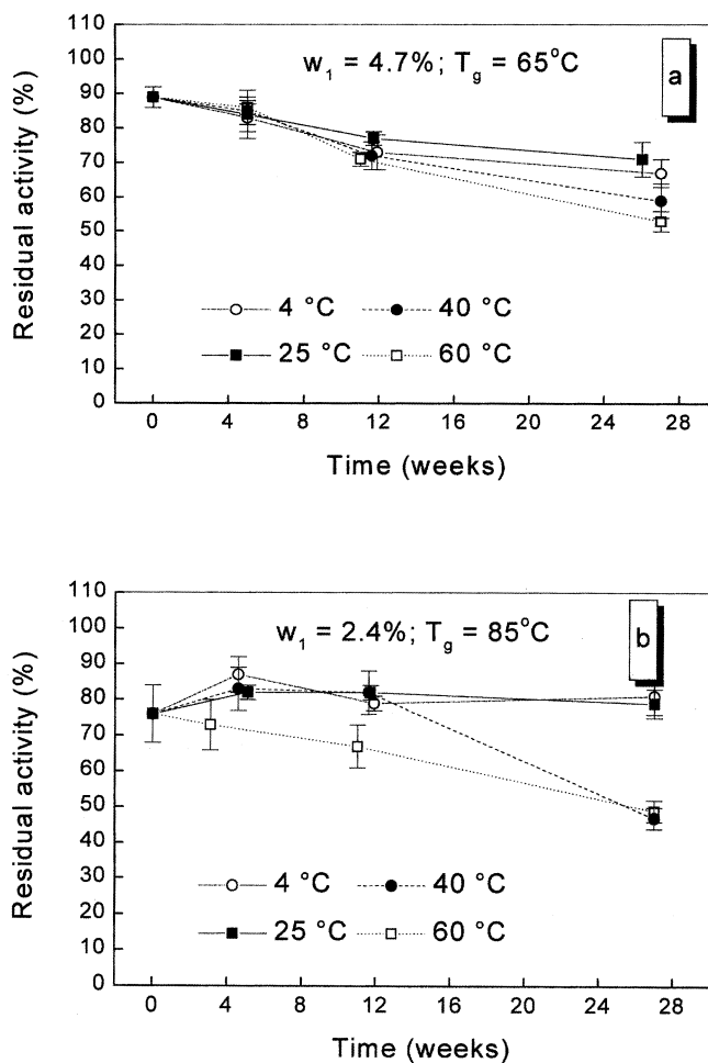
Figure 5. Residual activity of LDH measured immediately after spray-drying at T_{\text{inlet}}/T_{\text{outlet}} = (a) 90^\circ\text{C}/60^\circ\text{C} , or (b) 150^\circ\text{C}/95^\circ\text{C} , and also on subsequent dry-storage at various temperatures. Reproduced from Adler and Lee (1999) with permission.
