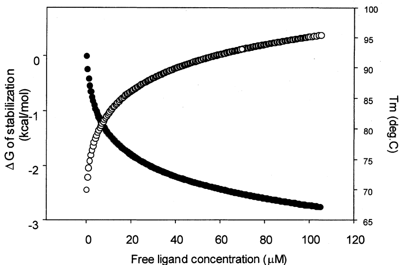
Figure 1. Hypothetical free energy of stabilization (filled circles) and corresponding increase in T_m (open circles) due to ligand binding to the native state ( K_n = 10^6 \text{ M}^{-1} ).
