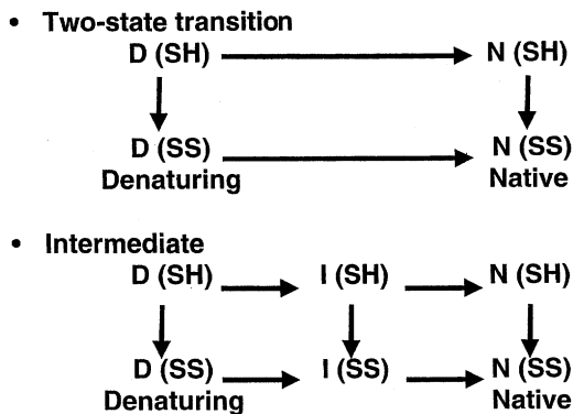
Figure 3. Refolding mechanism for proteins solubilized from inclusion bodies.
