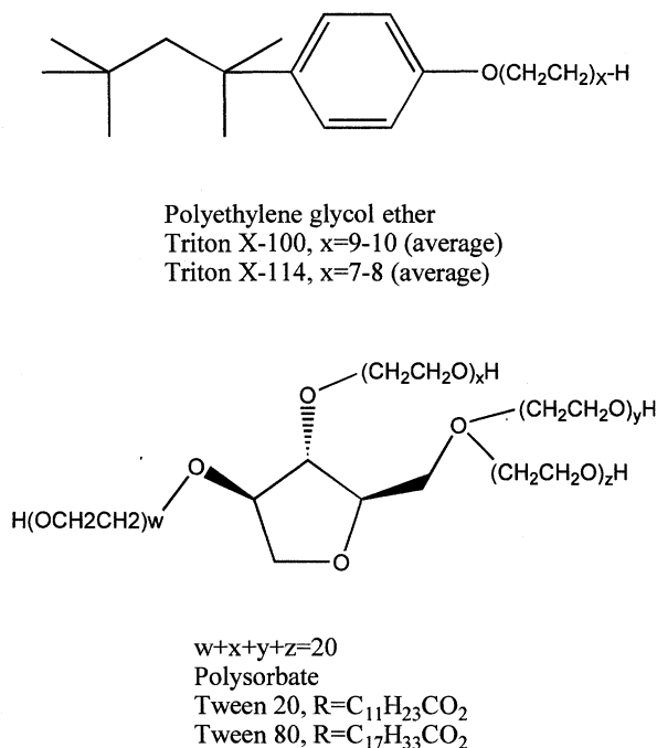
Figure 1. Example non-ionic surfactants.
