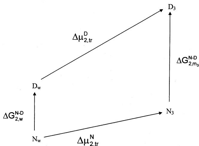
Figure a.4. Classical thermodynamic box for N to D transition in the presence and absence of an excluded cosolvent.
