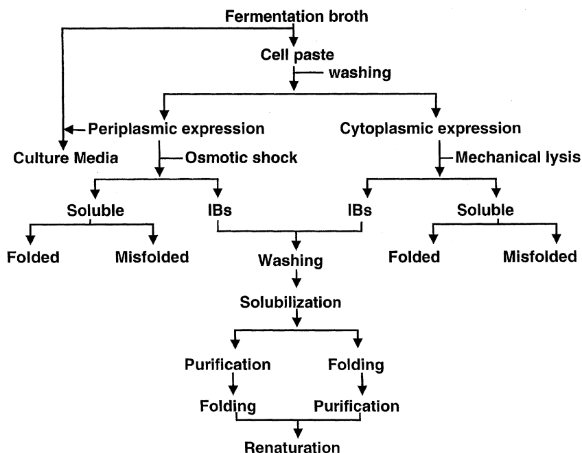
Figure 1. Distribution of recombinant proteins expressed in E. coli . IB's: inclusion bodies.
