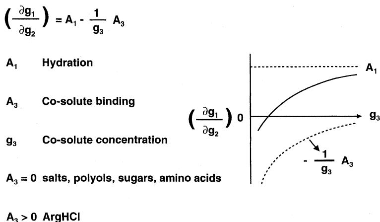
Figure 6. Schematic illustration of hydration and arginine-HCl binding to BSA used to interpret the observed preferential hydration of BSA in arginine-HCl shown in Figure 5.
