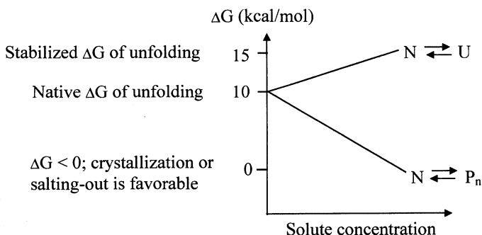
Figure a.2. Difference in \Delta G ( \Delta \Delta G ) of a process upon introduction of a cosolvent.
