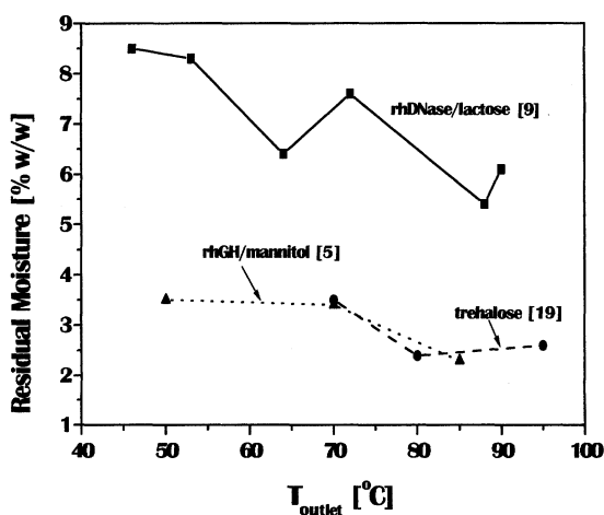
Figure 4. Relation between residual moisture and T_{\text{outlet}} for various spray-dried powders taken from the reference cited in the figure. The other independent process parameters ( v_{\text{lf}} , v_{\text{aa}} & v_{\text{da}} ) were not in all cases the same in the various works.
