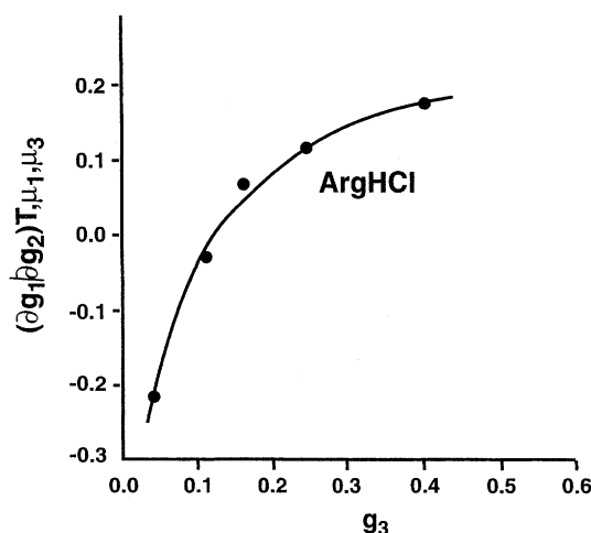
Figure 5. Preferential hydration of bovine serum albumin in arginine-HCl. Data taken from Arakawa and Timasheff, 1982b.
