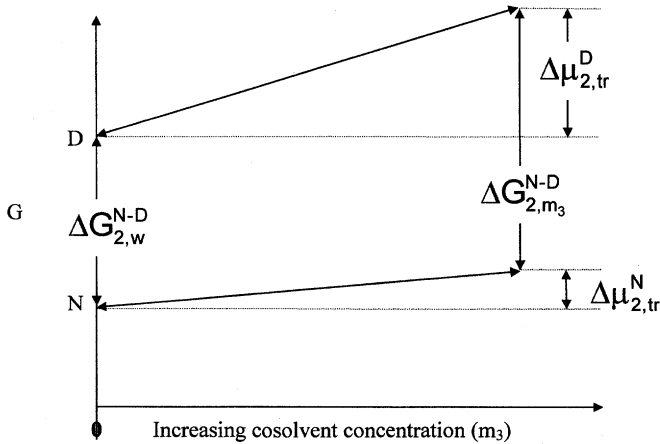
Figure a.3. Free energy of N to D transition in the absence and presence of an excluded cosolvent.
