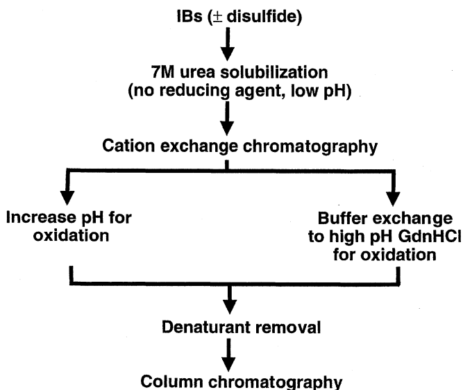
Figure 2. Generic purification protocol for recombinant proteins expressed in E. coli at inclusion bodies (IB's).
