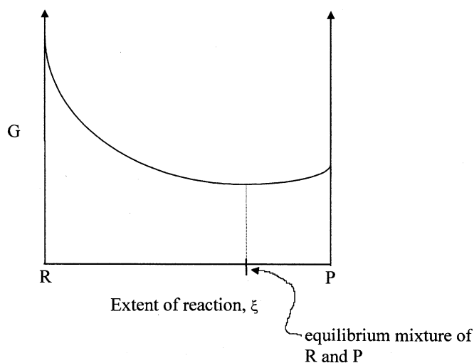
Figure a.1. Free energy of a reaction vs. extent of reaction.
