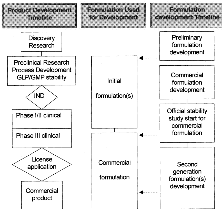
Figure 1. Diagram showing commercial formulation development process.
