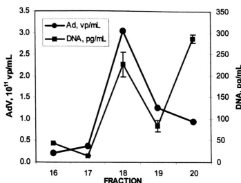
Figure 4. Second AEX chromatography on a purified product. Ad concentrations were measured by AEX HPLC and confirmed by A_{260} analysis. Residual DNA samples were measured in duplicate with mean and standard error reported.
