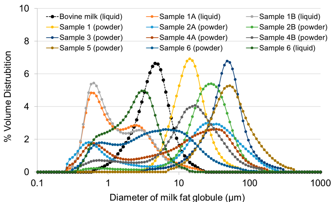
Figure 7. Size distribution of all liquid and powder WPPC samples from the data set and comparison with fresh raw bovine milk.
