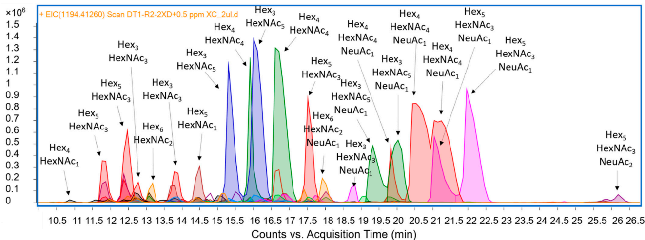
Figure 5. Overlaid extracted ion chromatograms of the most abundant WPPC N-glycans. The N-glycans are denoted by their monosaccharide compositions. Hex: hexose; HexNAc: N-acetylhexosamine; and NeuAc: N-acetylneuraminic acid.
