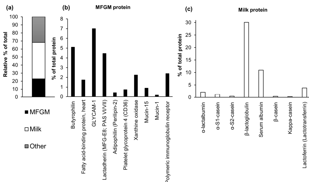
Figure 4. (a) Proteomics of whey protein phospholipid concentrate (WPPC), in which various protein abundances are expressed as a relative percentage of total protein. Proteins are divided into three groups: “MFGM proteins”, “milk proteins”, and “other proteins”. (b) Relative percentages of the milk fat globule membrane (MFGM) proteins in whey protein phospholipid concentrate (WPPC). (c) Relative percentages of milk proteins in whey protein phospholipid concentrate (WPPC).
