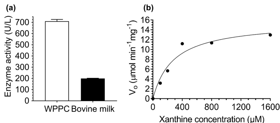
Figure 6. (a) Xanthine oxidase activity of whey protein phospholipid concentrate (WPPC) (sample 6B) and bovine milk, and (b) Michaelis–Menten kinetics of whey protein phospholipid concentrate (WPPC) xanthine oxidase for uric acid generation. For the graph, the corresponding fits (solid lines) K_m , and V_{max} data were obtained using the Michaelis–Menten equation.
