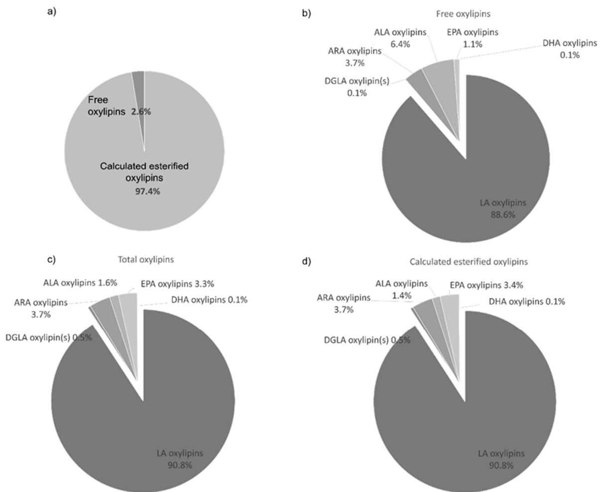
Figure 9. Pie charts listing the percentage distribution of (a) free vs. calculated esterified oxylipins (i.e., the difference between total and free oxylipins), (b) free oxylipins, (c) total oxylipins, and (d) calculated esterified oxylipins derived from various fatty acid precursors, including from linoleic acid (LNA), dihomogamma-linolenic (DGLA), arachidonic acid (ARA), \alpha -linolenic acid (ALA), eicosapentaenoic acid (EPA), and docosahexaenoic acid (DHA).
