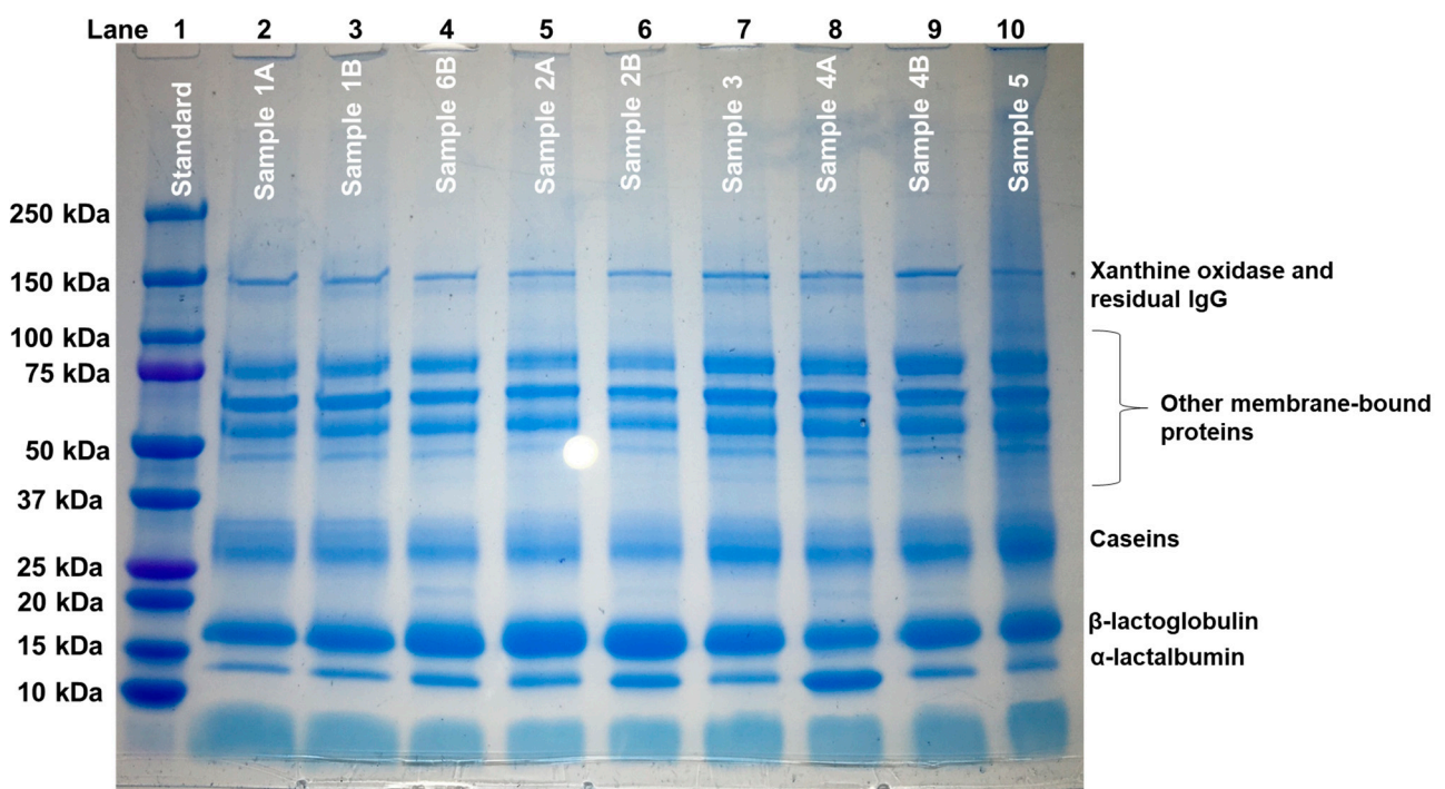
Figure 2. SDS-PAGE profile of whey protein phospholipid concentrate (WPPC) from different manufacturers. Lane 1: standard; Lane 2: sample 1A; Lane 3: sample 1B; Lane 4: sample 6B; Lane 5: sample 2A; Lane 6: sample 2B; Lane 7: sample 3; Lane 8: sample 4A; Lane 9: sample 4B; and Lane 10: sample 5. Annotation based on [57] with the exception of xanthine oxidase and IgG.
