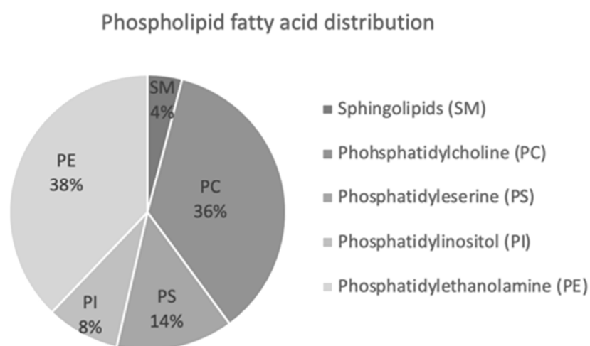
Figure 8. Phospholipid fraction distribution (calculated based on fatty acid composition per each fraction).
