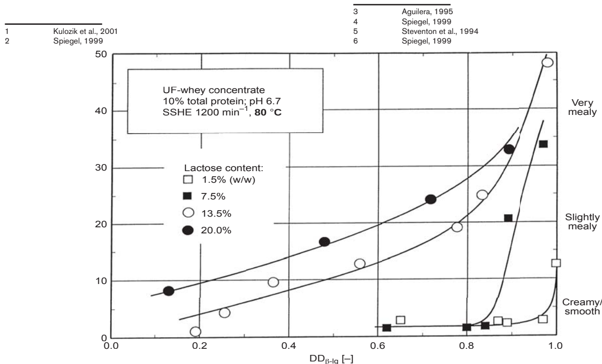
Fig. 4: Effect of the degree of denaturation of \beta -lg on the aggregate size (Spiegel, 1999)
