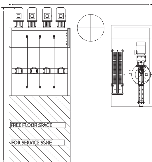
Fig.15: Dimentional sketch of APV LeanCreme™ plant with capacity of 1,500 l/h
