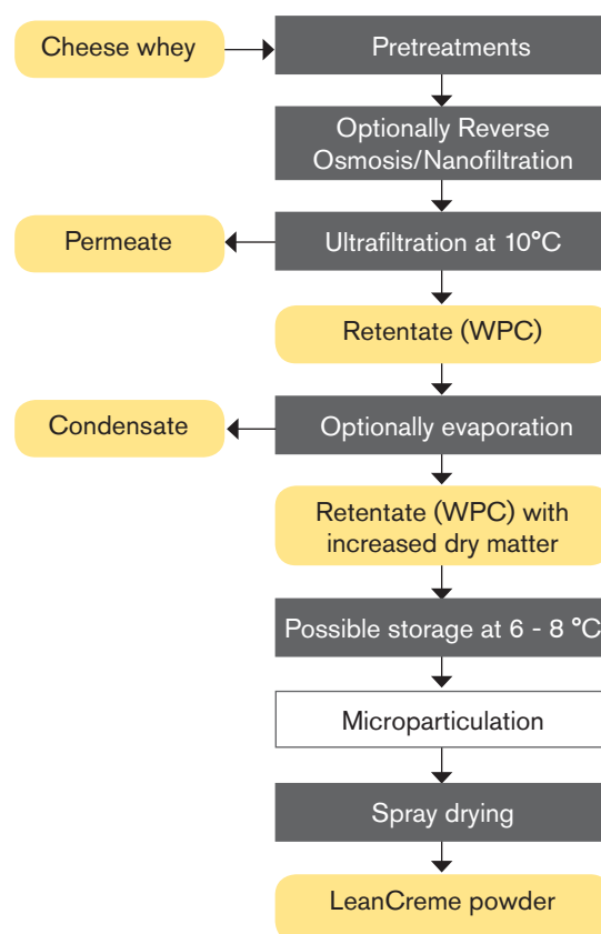
Fig. 18: Diagram of manufacturing of LeanCreme powder treated by the APV LeanCreme™ process including cooling to 50°C. The LeanCreme can proceed directly to the spray dryer. Fig. 18 shows a diagram of the process.
