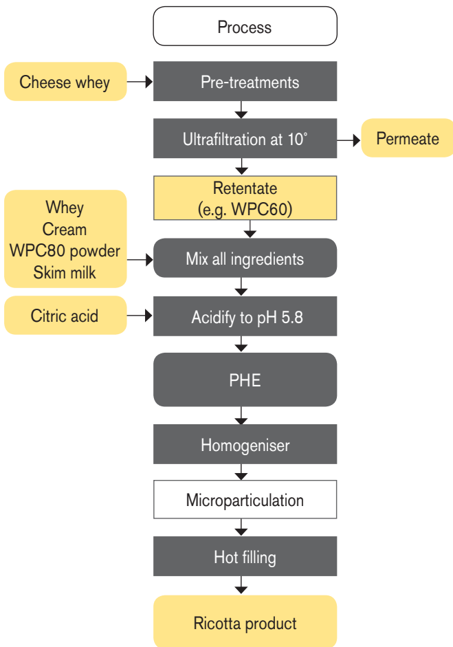
Fig. 19: Diagram of manufacturing Ricotta and similar products
