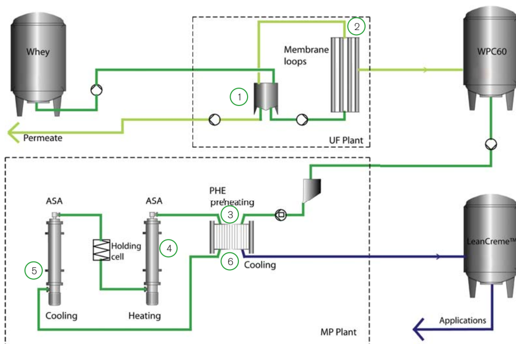
Fig. 11: The APV LeanCreme™ process
