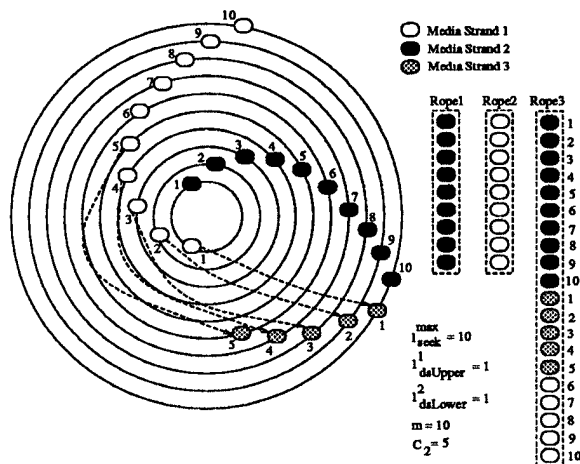
Figure 10: Copying of strands in editing operations (Rope3 \leftarrow CONCATE[Rope1, Rope2])
