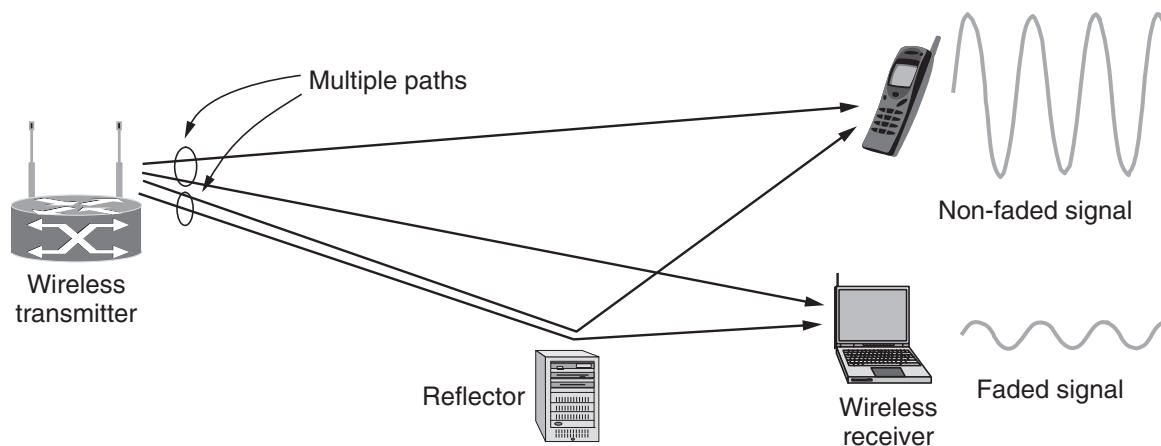
Figure 1-34. Multipath fading.
