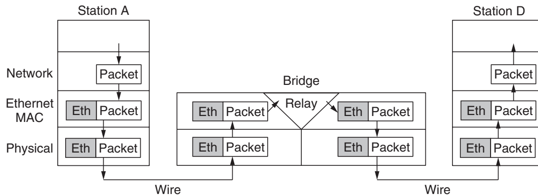
Figure 4-42. Protocol processing at a bridge.
