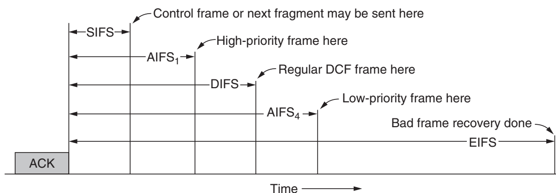
Figure 4-28. Interframe spacing in 802.11.
