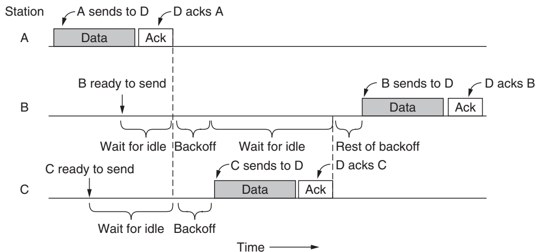
Figure 4-25. Sending a frame with CSMA/CA.
