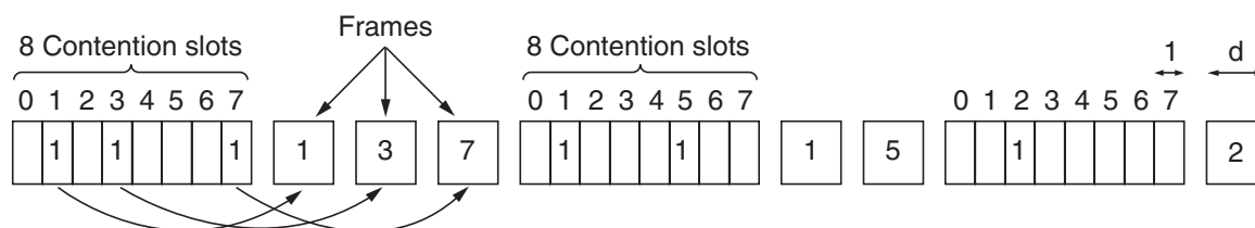
Figure 4-6. The basic bit-map protocol.
