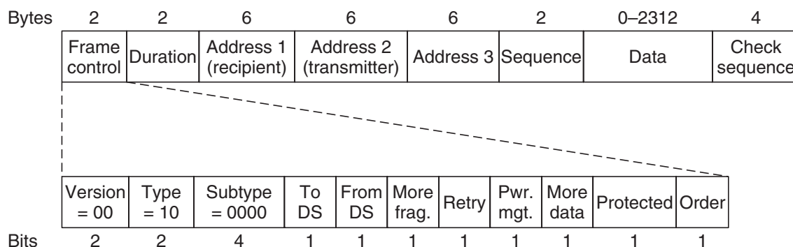
Figure 4-29. Format of the 802.11 data frame.
