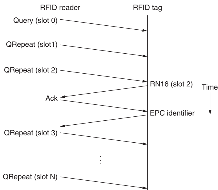
Figure 4-39. Example message exchange to identify a tag.
