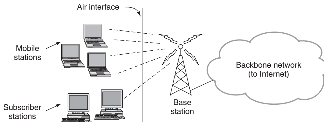
Figure 4-30. The 802.16 architecture.
