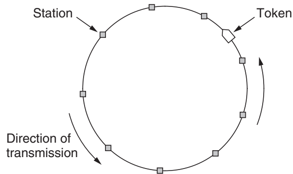
Figure 4-7. Token ring.
