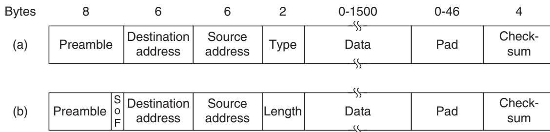
Figure 4-14. Frame formats. (a) Ethernet (DIX). (b) IEEE 802.3.
