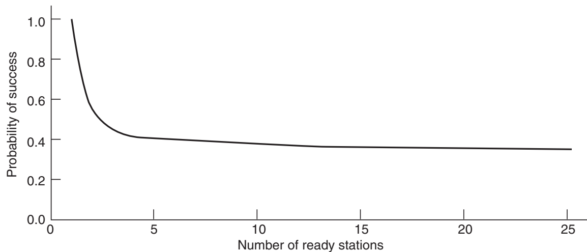
Figure 4-9. Acquisition probability for a symmetric contention channel.
