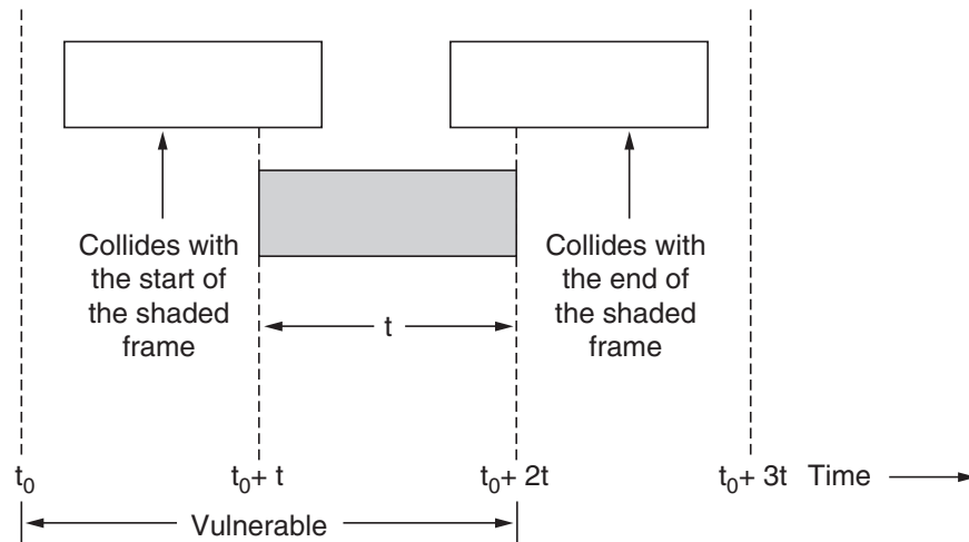
Figure 4-2. Vulnerable period for the shaded frame.
