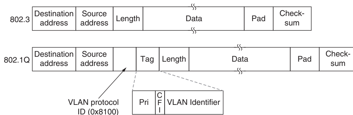
Figure 4-49. The 802.3 (legacy) and 802.1Q Ethernet frame formats.
