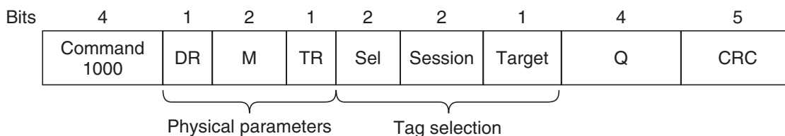
Figure 4-40. Format of the Query message.
