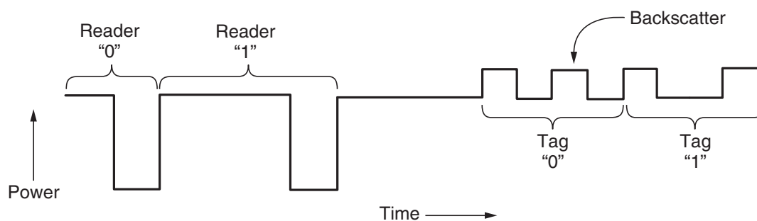
Figure 4-38. Reader and tag backscatter signals.
