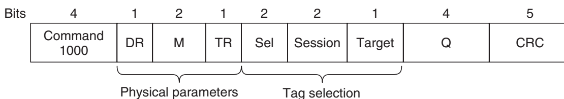
Figure 4-40. Format of the Query message.
