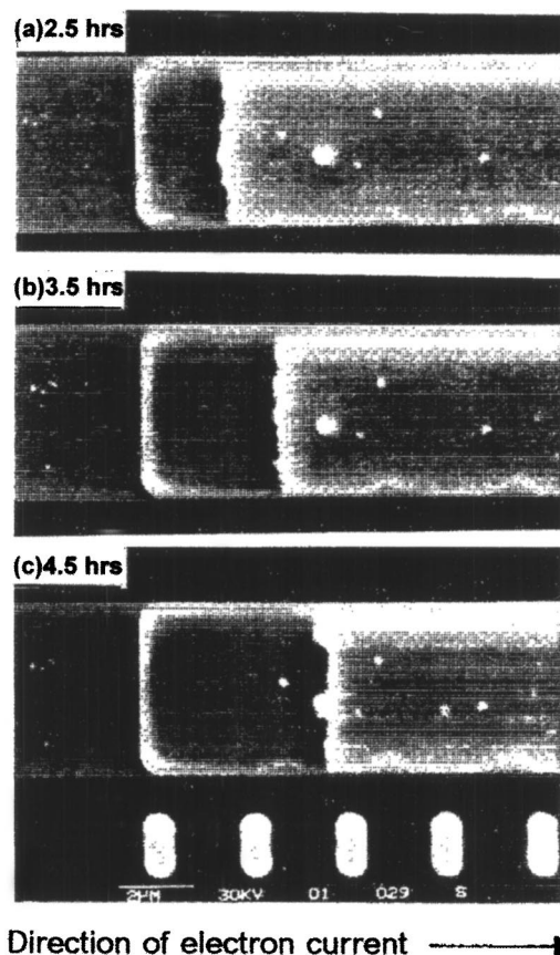
FIG. 4. (a) SEM image of mass depletion at cathode of a Cu strip at 2.5 h at 400 °C with current density of 2.1 \times 10^6 A/cm 2 , (b) at 3.5 h, and (c) at 4.5 h. The drift velocity is about 2 \mu m/h as measured from the three images (Ref. 13).
