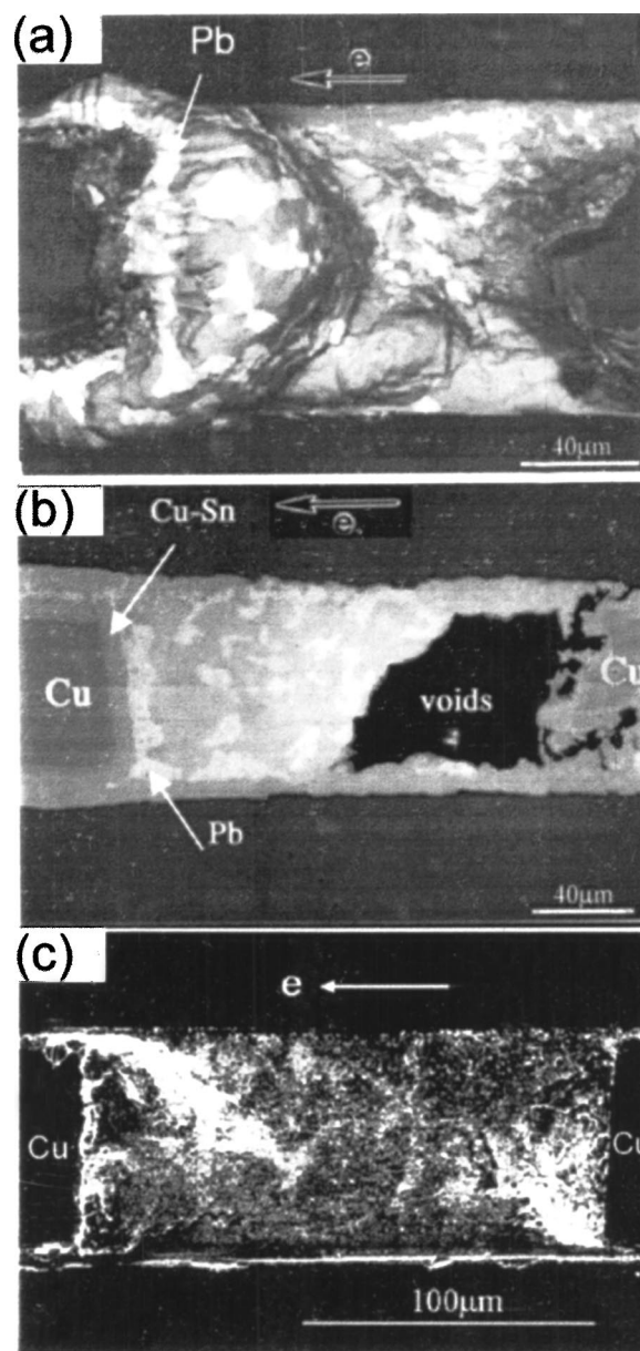
FIG. 22. SEM images of morphological changes on a eutectic SnPb solder line due to electromigration: (a) large lump formation at the anode after applying 2.8 \times 10^4 \text{ A/cm}^2 at 150 °C for 8 days; (b) void at the cathode in a top-down cross section of the sample shown in (a); and (c) a sample at room temperature with 5.7 \times 10^4 \text{ A/cm}^2 for 12 days (Refs. 57 and 62).
