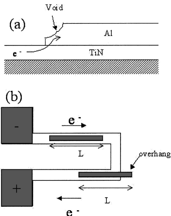
FIG. 27. (a) Schematic diagram of the cross section of an Al short strip on TiN and the formation of a void at the upper-left corner where current density is low. (b) Schematic diagram of the top view of a TiN base line having a U-turn and an Al short strip having an overhang (Refs. 74 and 75).
