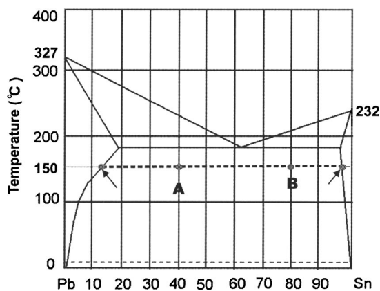
FIG. 20. Schematic binary eutectic phase diagram of Sn–Pb. Along the broken line at constant 150^\circ\text{C} , there is no chemical potential change as a function of composition. Hence, we can have phase separation along the broken line driven by electromigration.
