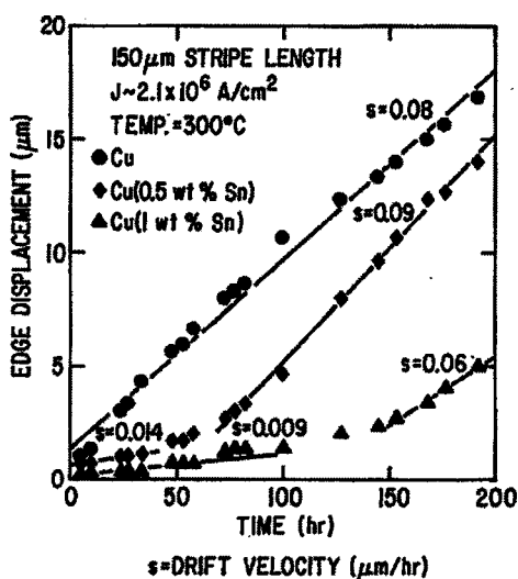
FIG. 12. Plots to show the comparison of edge displacements vs time for 150-μm-long strips of Cu and Cu(Sn) alloys at 300 °C with current density of 2.1 \times 10^6 A/cm 2 . The measured drift velocity "s" is given in the figure (Ref. 13).
