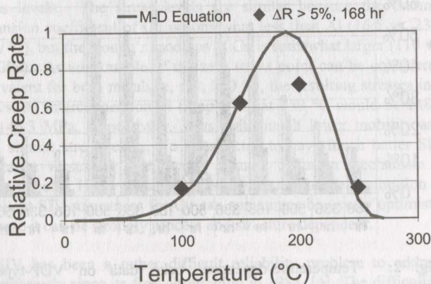
Fig. 3: McPherson and Dunn creep/voiding rate model.
