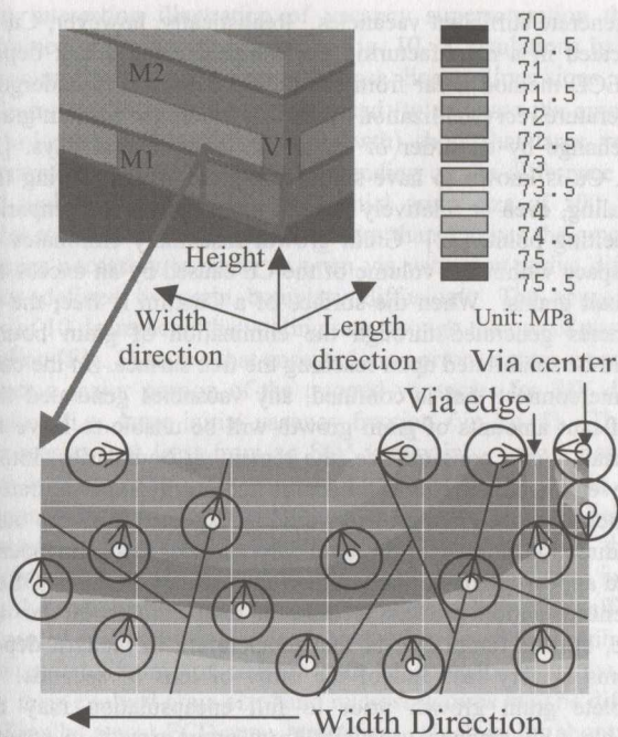
Fig. 8: Finite Element Analysis of dual-damascene via placed over a wide metal lead. Hydrostatic stress contours are shown. Via diameter is 0.18 \mu\text{m} . A local region of higher tensile stress is found directly underneath the via center. A local region of lower tensile stress is exhibited under the edge of the via. These two regions of stress concentration lead to a prominent stress gradient under the via that drives vacancies under the via towards its bottom perimeter. Smaller compressively directed stress gradients exist around the via perimeter from both below and horizontally just outside the via edge. A small, white sphere (circle in two-dimensions) with an arrow that extends from its center and terminates at the boundary of a greater sphere is meant to illustrate the diffusional process and is called a “diffusion sphere.” The white circle represents a vacancy. The arrow denotes the general direction of vacancy motion – in a statistical sense – under a stress gradient driving force. The arrow is oriented normally to the surface contour of constant stress – unless somehow constrained – and is directed from a region of higher to lower stress. The greater circle represents how far a given vacancy will travel, d , within a specific time interval, \Delta t , according to some diffusional mechanism, D , where d \sim \sqrt{(D\Delta t)} . The fine solid lines show how grain boundaries might be overlaid over the stress profile, which would also form a constraining pathway for vacancy migration along the boundary. As depicted above, vacancies are migrating along a number of pathways and, depending on the transport mechanism, the diffusion spheres generally would be differently size for a fixed time interval \Delta t ; however, for visual clarity and simplicity, they are drawn identically.
