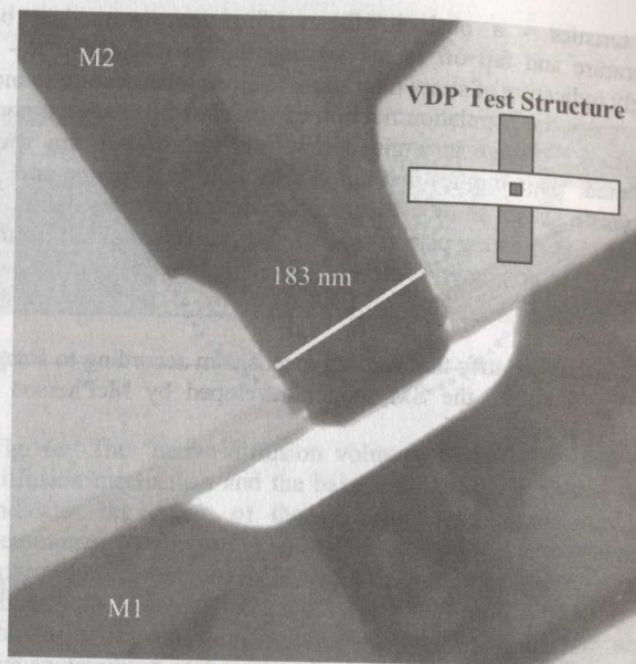
Fig. 1: Void-formation under a small via placed over a wide metal lead. The M1 lead is about 3 \mu\text{m} wide. The void was formed after baking for over 100 hrs. at 150^\circ\text{C} . The inset graphic shows the basic characteristics of the test structure.
