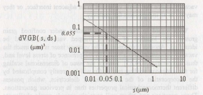
Fig. 10: Void volume calculated assuming grain size doubling in a constrained interconnect. s = initial grain size, \mu\text{m} ; ds = 0.0005 \mu\text{m} = grain boundary width; dVGB(s, ds) = Total void volume generated by GB elimination for grains sizes up to the active interconnect volume; V_{\text{Cu,Active}}(150^\circ\text{C}, 100 \text{ hr}) \sim 3.7 \mu\text{m}^3 .
