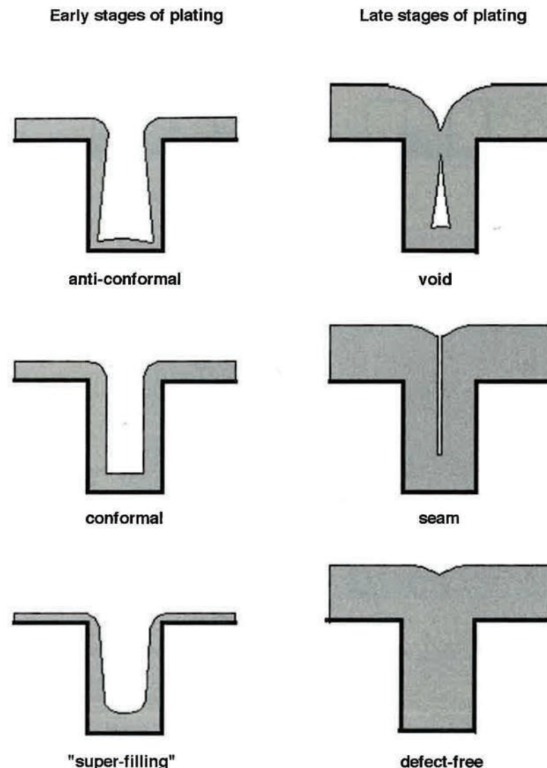
FIG. 4. Types of profile evolution in Damascene plating (Copyright 1998 International Business Machines Corporation. Reprinted with permission of the IBM Journal of Research and Development, Volume 42, Number 5.)
