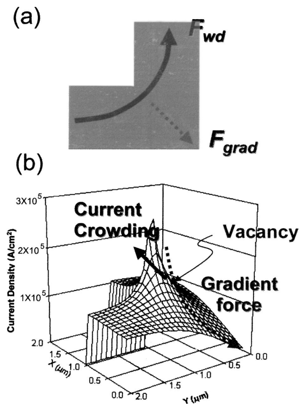
FIG. 29. (a) Schematic diagram of a 90° turn in an interconnect, where F_{wd} is electron wind force and F_{grad} is current density gradient force. (b) Current density distribution in the 90° turn, in which current crowding occurs at the inner corner (Ref. 76).
