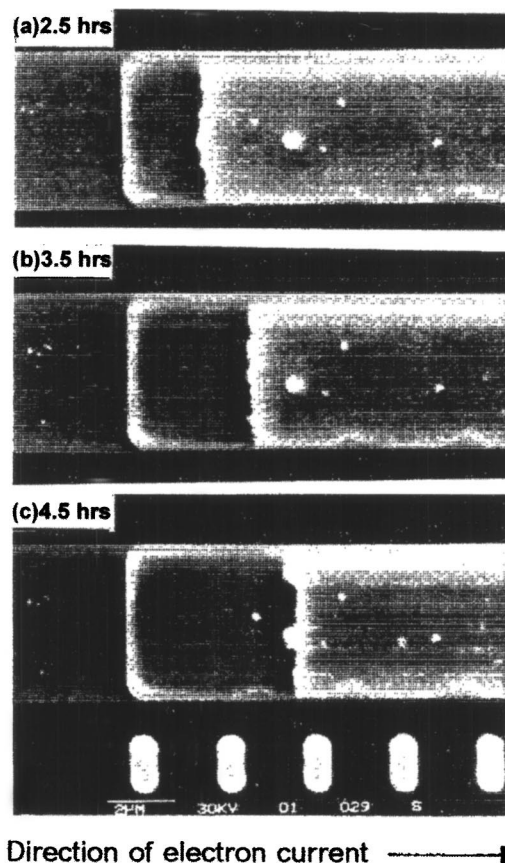
FIG. 4. (a) SEM image of mass depletion at cathode of a Cu strip at 2.5 h at 400 °C with current density of 2.1 \times 10^6 A/cm 2 , (b) at 3.5 h, and (c) at 4.5 h. The drift velocity is about 2 μm/h as measured from the three images (Ref. 13).
