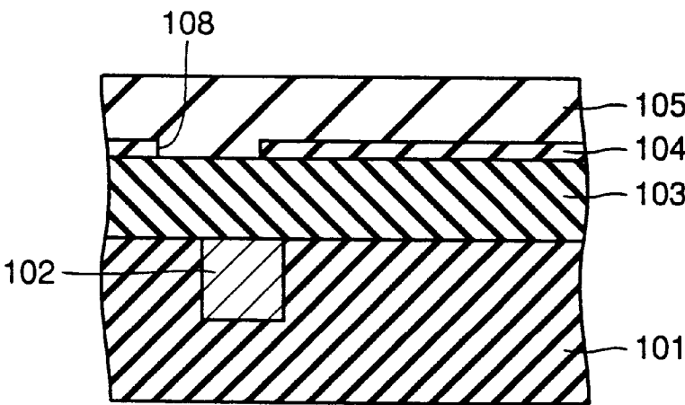
FIG. 22 PRIOR ART
