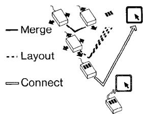
Fig. 2. Composition operators used in describing the mouse
