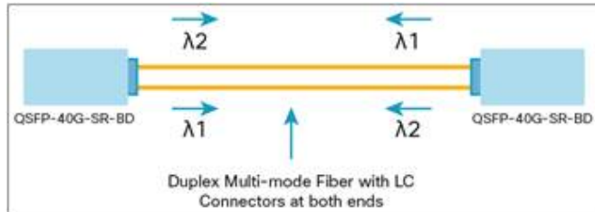
Figure 1. Cisco QSFP BiDi 40Gbps Transceiver: Duplex MMF with LC Connectors at Both Ends
