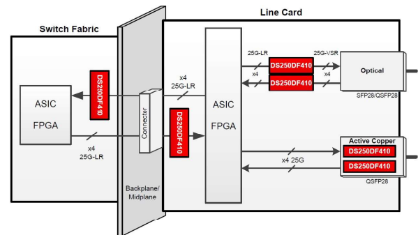
Fig. 3.0: Typical Uses for the retimer in a system.
