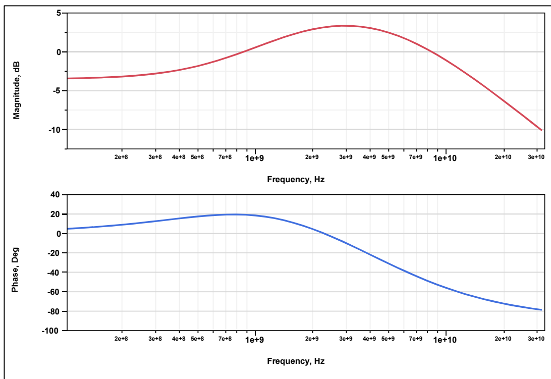
Figure 5 An illustrative example of the amplitude and phase Bode plots of a CTLE equalizer. A specific re-driver's CTLE is usually different from the above, depending on the design and bitrate. Notice the nonlinear phase response (versus frequency) of this 1-zero 2-pole equalizer.
