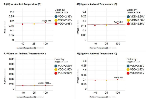
Fig. 13.0: Output jitter over voltage and temperature.
