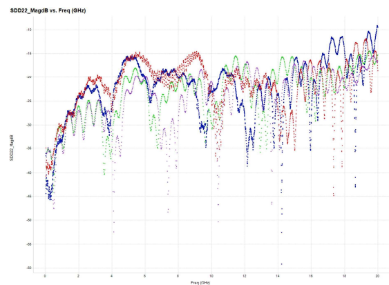
Fig. 15.0: Simulation to measurement correlation for 2 channels.
