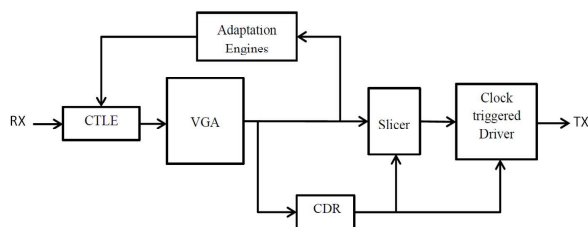
Fig. 1.0: Typical components of a retimer implementation.
