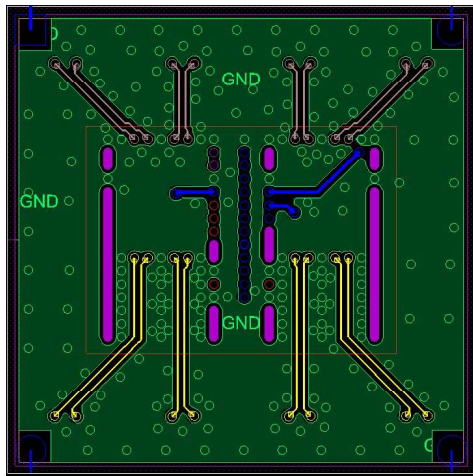
Fig. 4.0: Top view of package design for the device.
