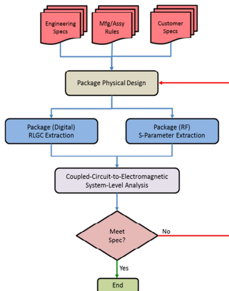
Fig. 9.0: System co-design modeling methodology and flow.
