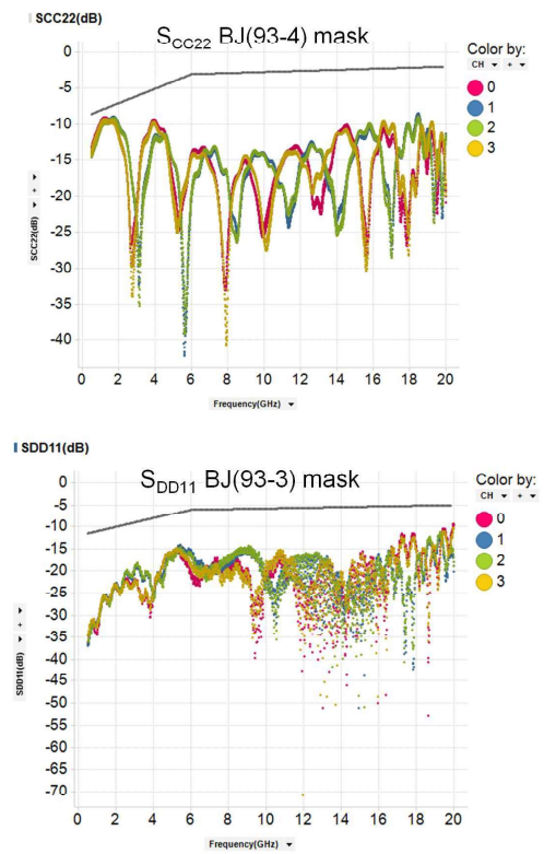
Fig. 11.0: Sample TX and RX return loss measurements.
