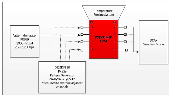
Fig. 12.0: Test set-up for measuring output jitter.
