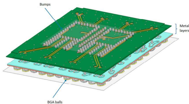
Fig. 5.0: 3D view of the package design for the device.
