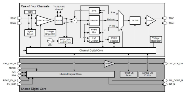
Fig. 2.0: Functional block diagram of the retimer.
