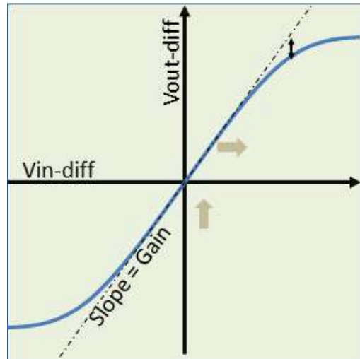
Figure 11 Relationship between the input and output amplitudes of a “Linear” re-driver, showing linearity over a certain input range, and the eventual onset of saturation (or compression).
