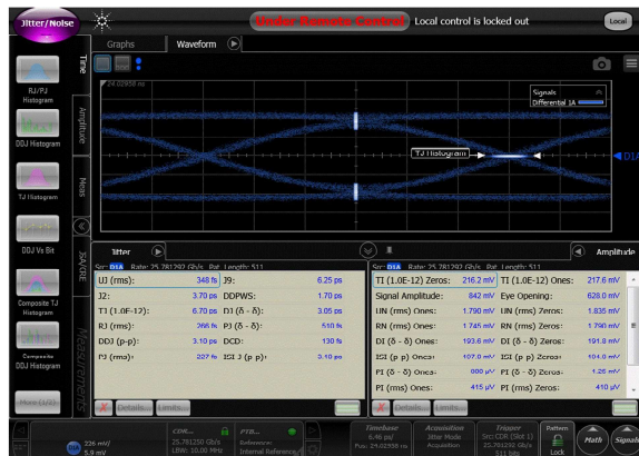
Fig. 14.0: Eye diagram under typical conditions.
