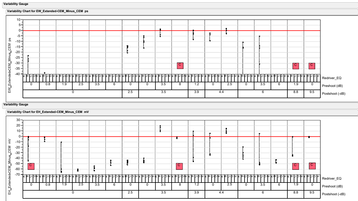
Figure 28 The difference between the EW of the CEM+8dB (@4GHz) of total extension and the “Ref. CEM channel” alone, using a second re-driver offering, vs. the range of TxEQ values selected in Figure 21. Only the most relevant re-driver setting is shown here. Note how no one re-driver setting produces a positive (or zero) delta at all TxEQs. The red boxes indicate closed Ref. CEM eyes using the Ref. receiver.
