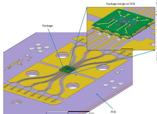
Fig. 8.0: 3D view of merged Package and PCB physical designs for accurate 3D modeling and extraction.
