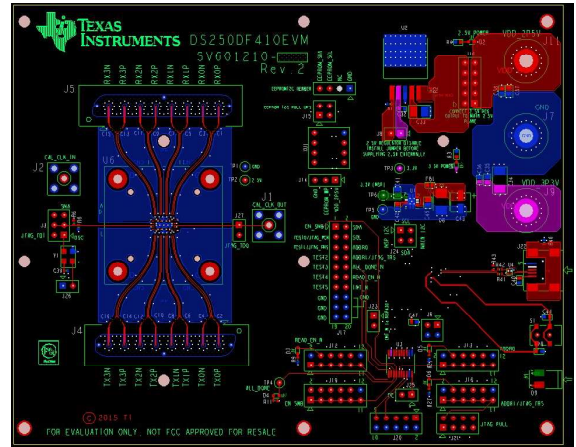
Fig. 6.0: Top view of the EVM PCB design for the device.
