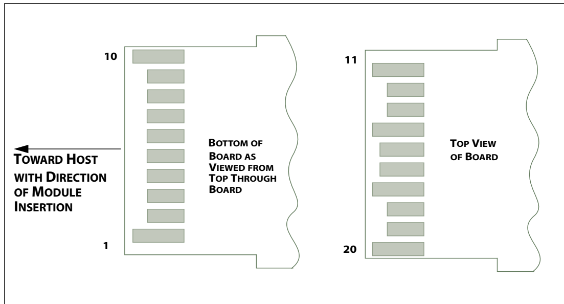
Figure 2 SFP+ module contact assignment
