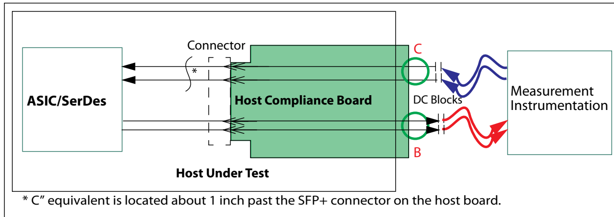
Figure 13 Host Compliance Board
