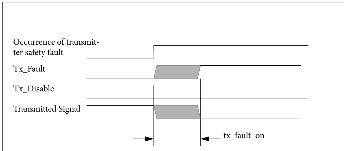
Figure 7 Occurrence of condition generating Tx_Fault
