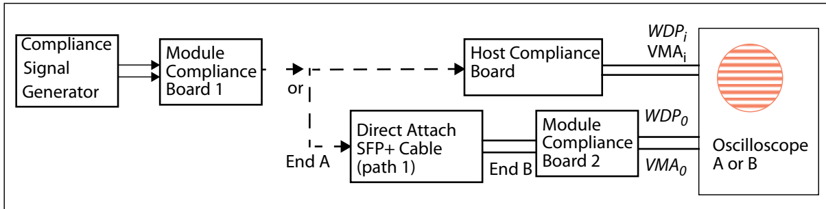
Figure 64 10GSFP+Cu Cable NEXT dWDP Test Setup
