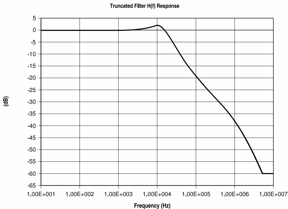
Figure 57 Reference filter response
