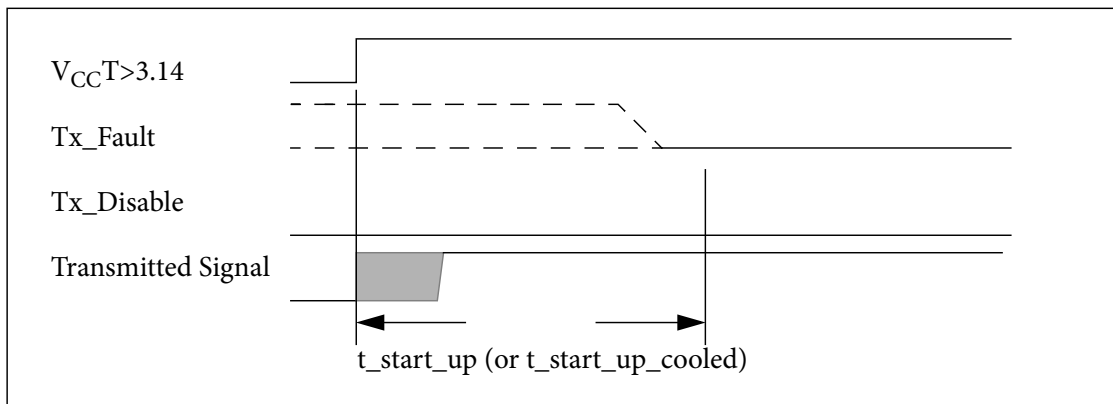
Figure 3 Power on initialization of module, Tx_Disable negated
