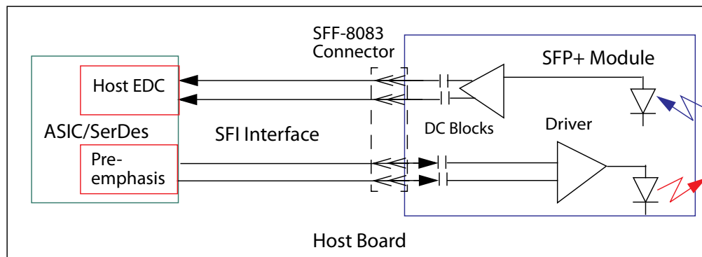
Figure 12 SFI Application Reference Model
