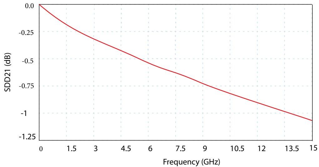
Figure 35 Approximate Transfer Response of Module Compliance Board
