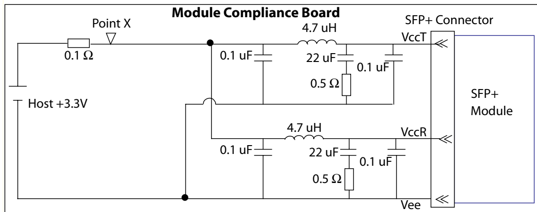
Figure 56 Module Compliance Board Power Supply Filters
