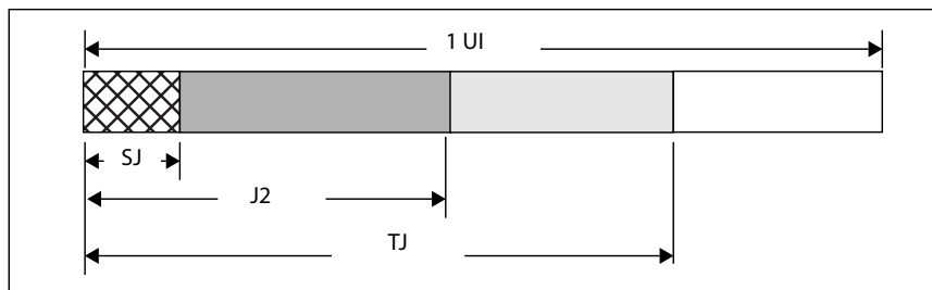
Figure 51 Stressed eye jitter components
