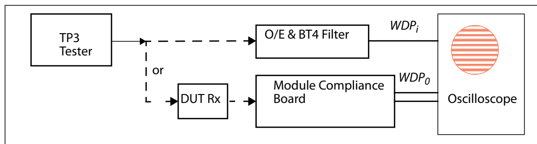
Figure 54 Module receiver waveform penalty compliance test
