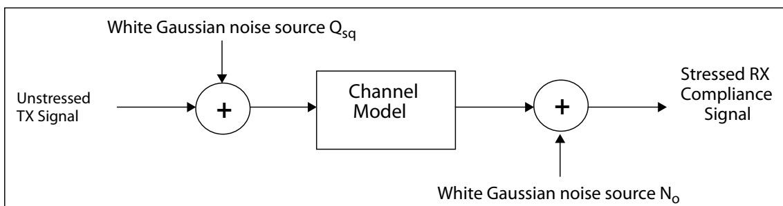
Figure 61 Block Diagram of Copper Stressor Noise Model
