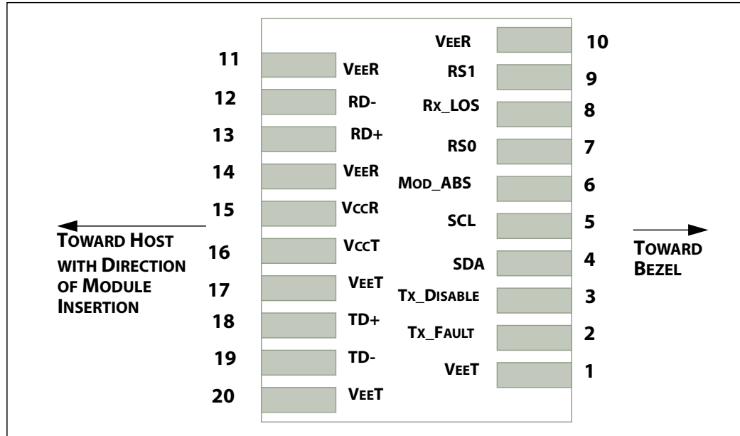
Figure 1 Host PCB SFP+ pad assignment top view
