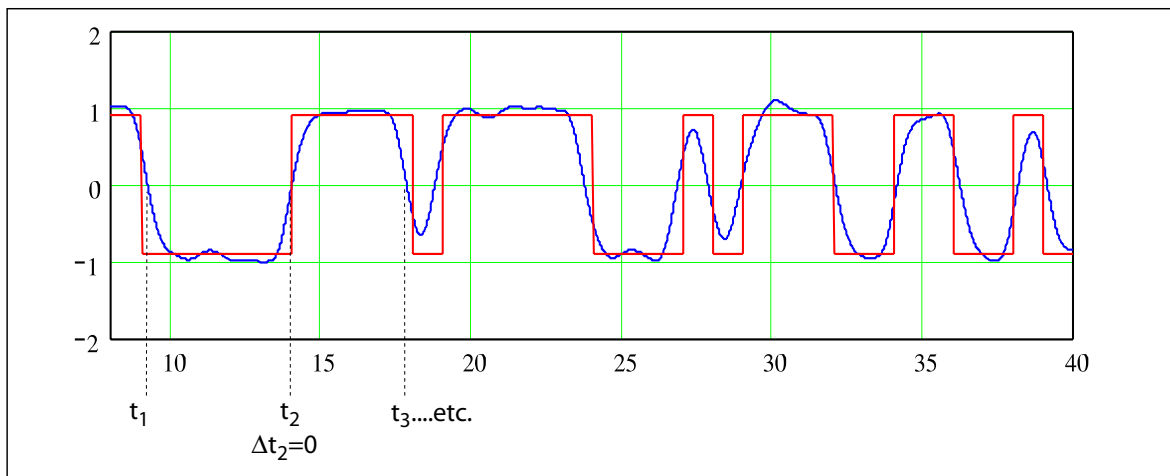
Figure 47 DDJ Test Method
