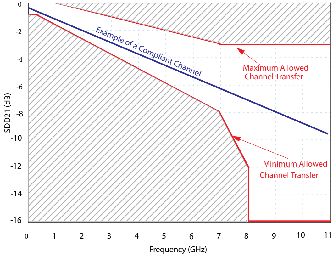
Figure 33 Example of SFI Host Recommended Channel
