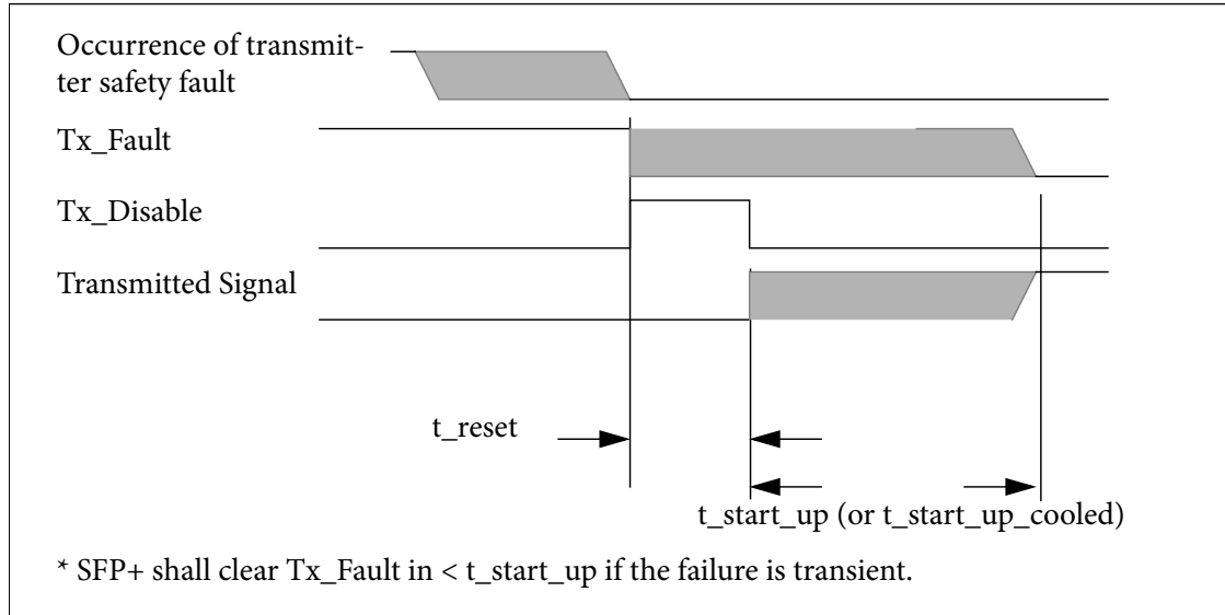
Figure 8 Successful recovery from transient safety fault condition
