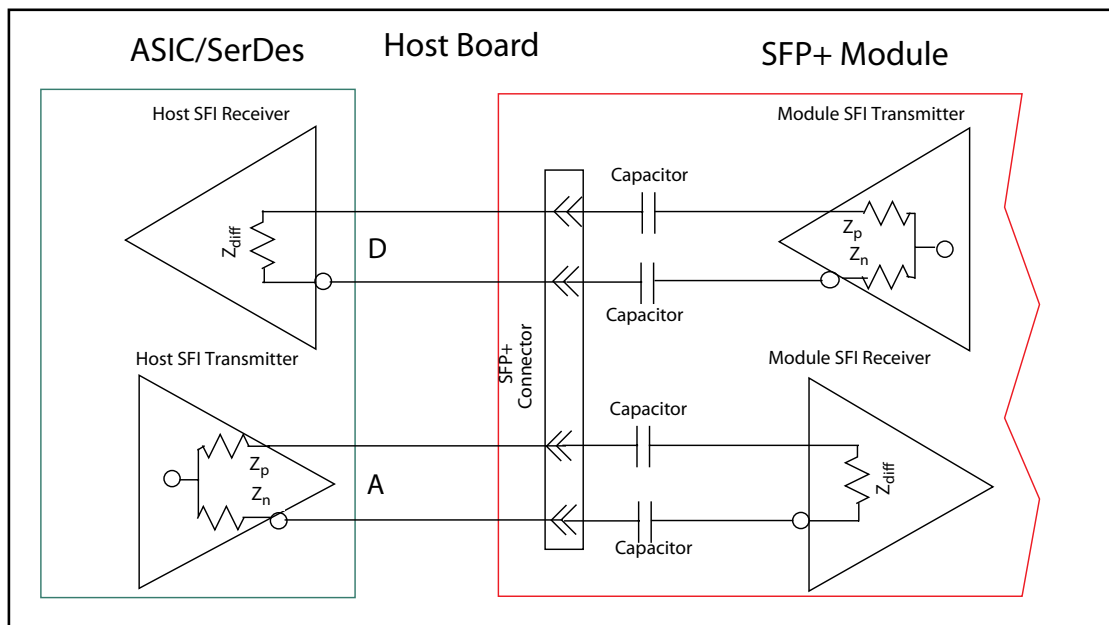
Figure 18 SFI Termination and AC Coupling
