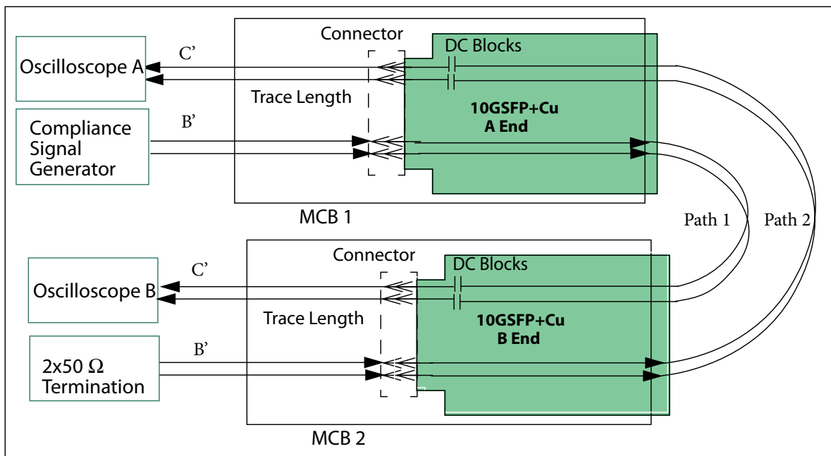
Figure 63 10GSFP+ Cable Test Setup
