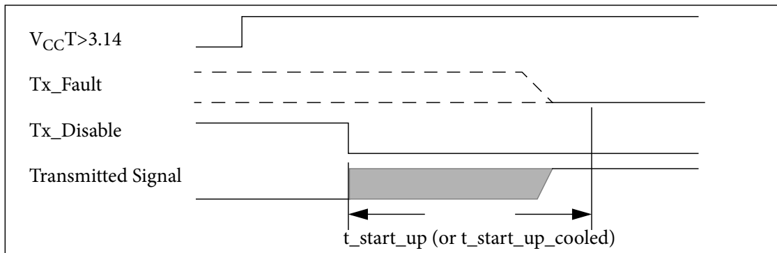
Figure 4 Power on initialization of module, Tx_Disable asserted
