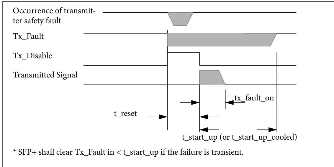
Figure 9 Unsuccessful recovery from safety fault condition
