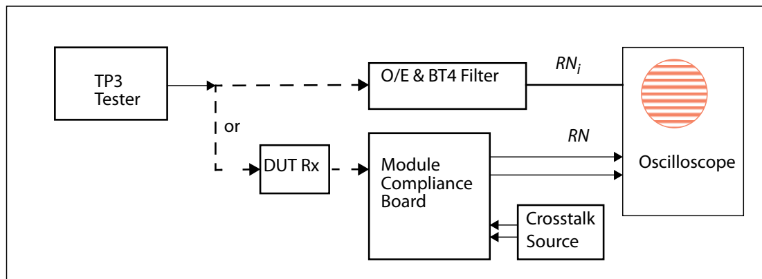
Figure 53 Linear Module Receiver Noise Test
