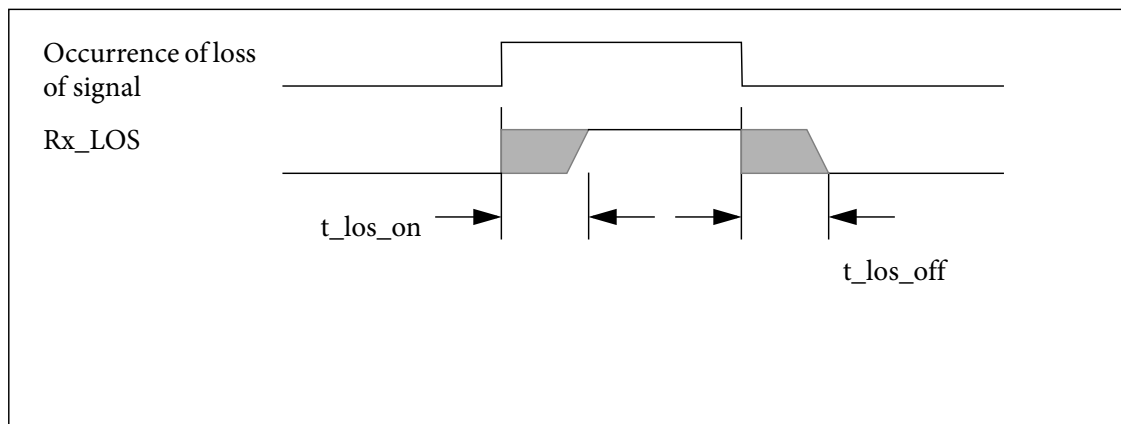
Figure 10 Timing of Rx_LOS detection
