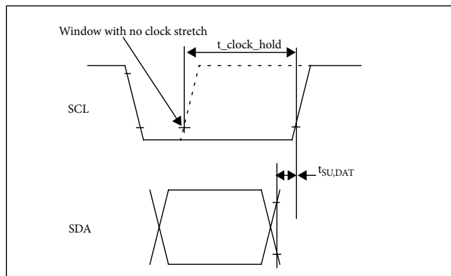
Figure 25 2-wire Timing Diagram
