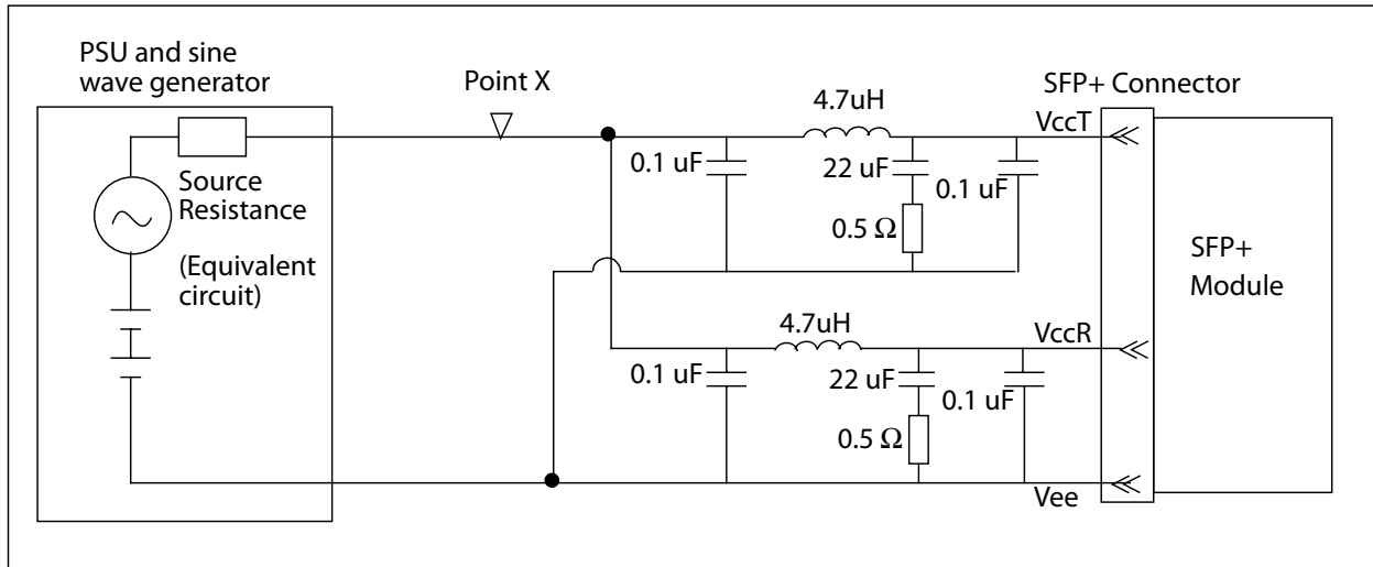
Figure 58 Power Supply Noise Tolerance Test Setup
