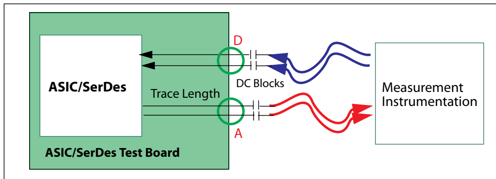
Figure 15 ASIC/SerDes Test Board
