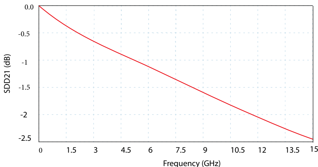
Figure 34 Approximate Response of Host Compliance Board
