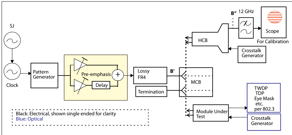
Figure 49 Compliance signal generator for module transmitter
