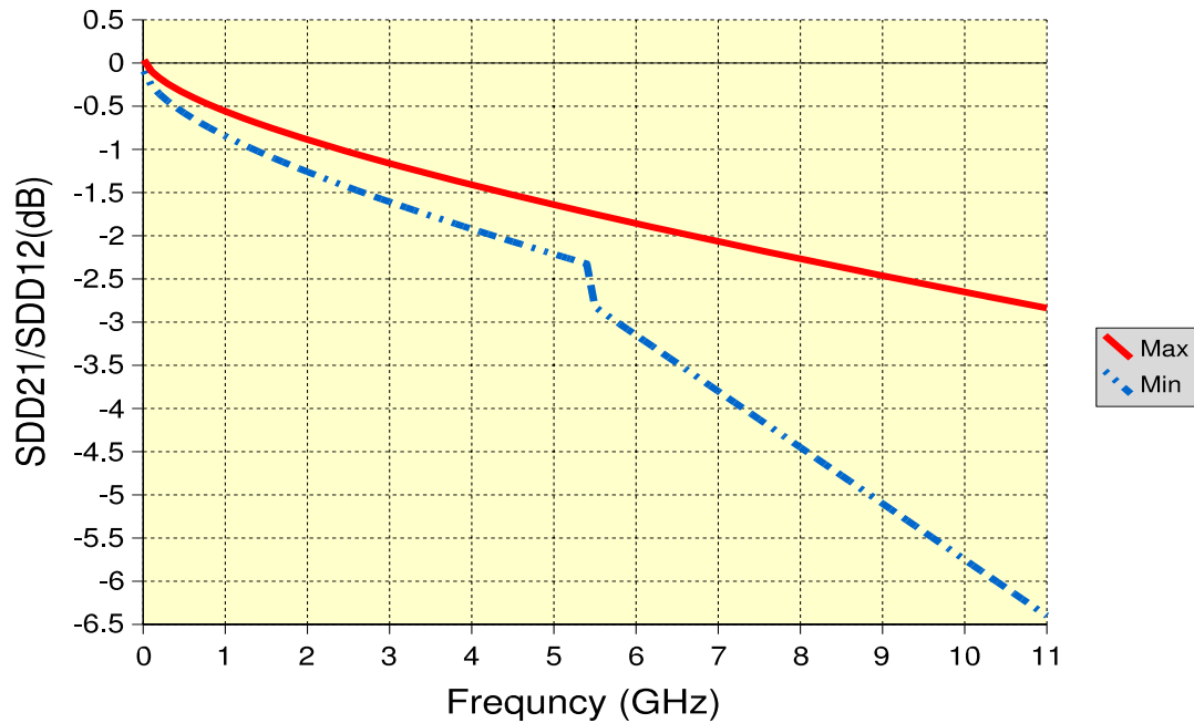
Figure 42 Mated MCB-HCB Differential Through Response Limits
