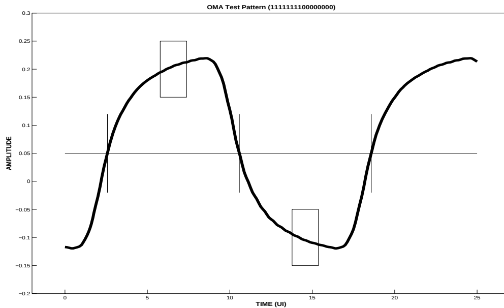
Figure 48 Example xMA waveform showing xMA measurement windows
