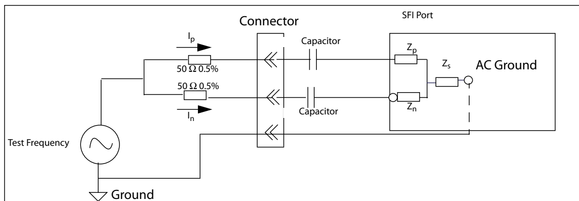
Figure 55 AC Termination Mismatch Measurement
