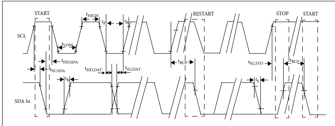
Figure 25 2-wire Timing Diagram
