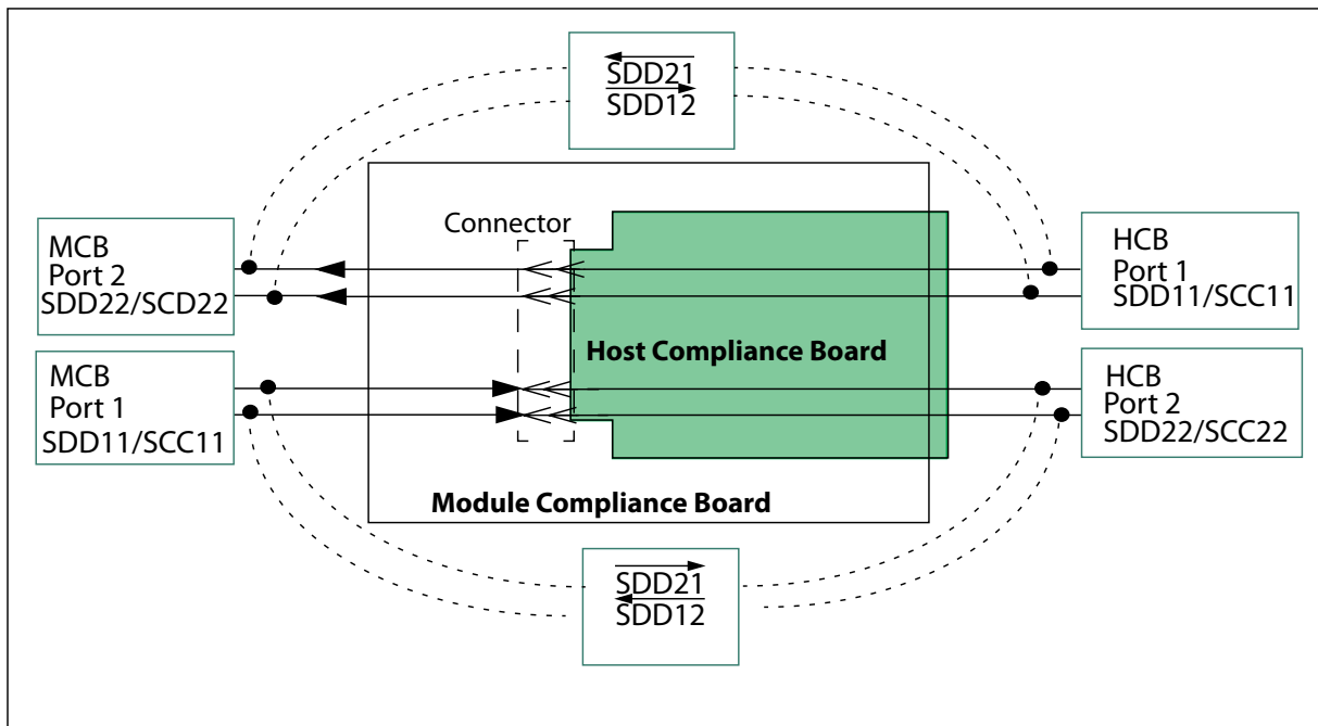
Figure 40 Measurements Port Definition
