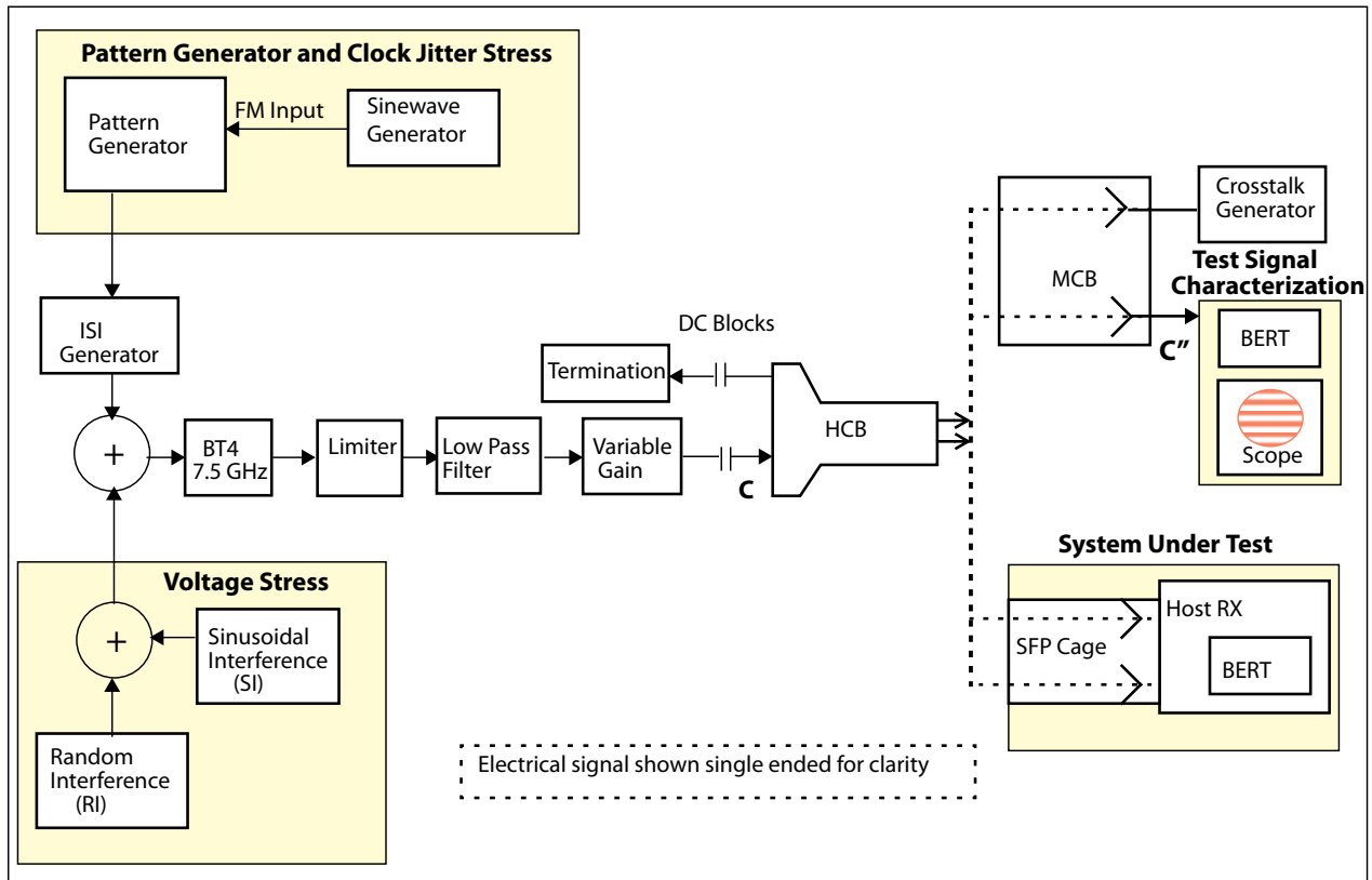
Figure 50 Jitter Tolerance Test Configuration
