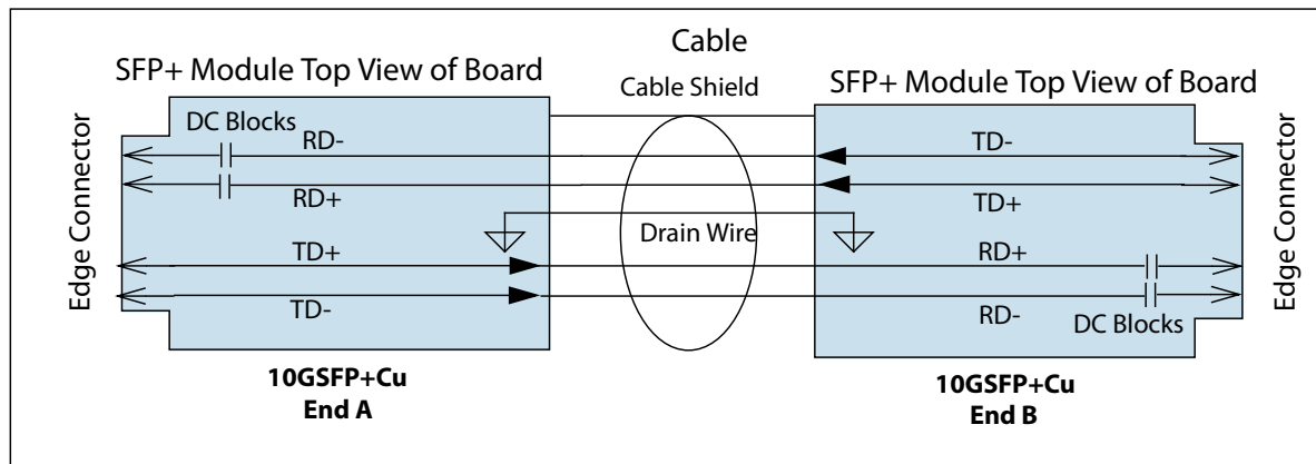
Figure 59 10GSFP+Cu Direct Attach Block Diagram
