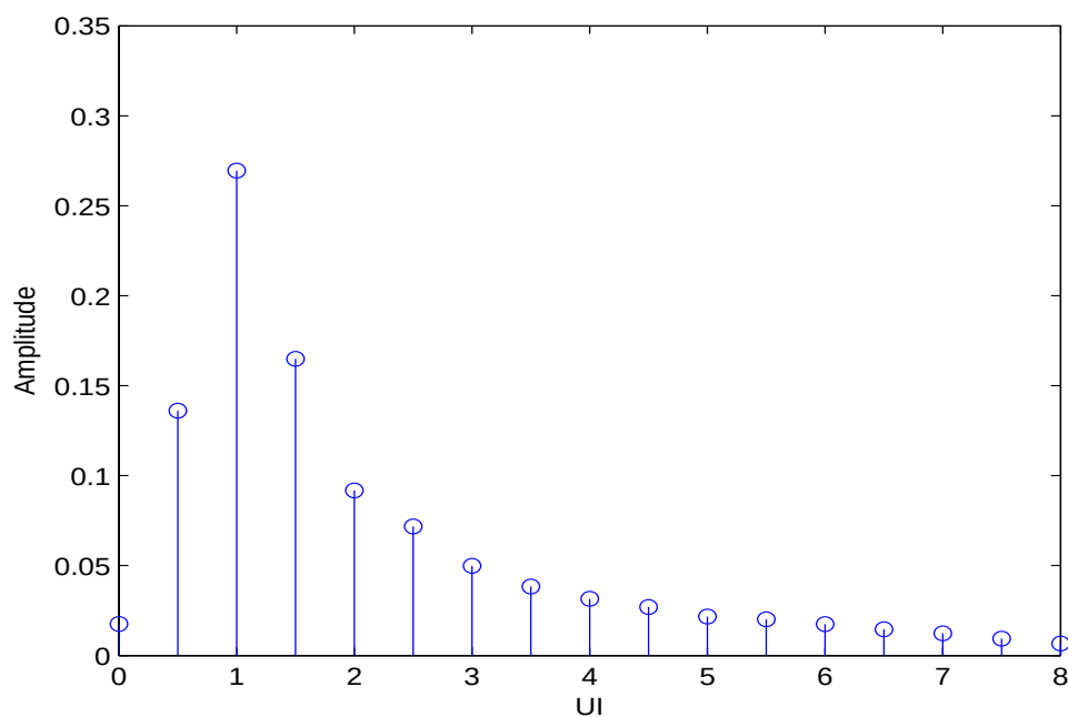
Figure 60 10GSFP+Cu TWDPc Stressor Impulse Response
