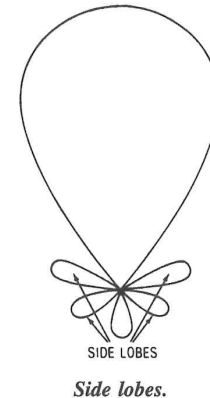
Side lobes.
