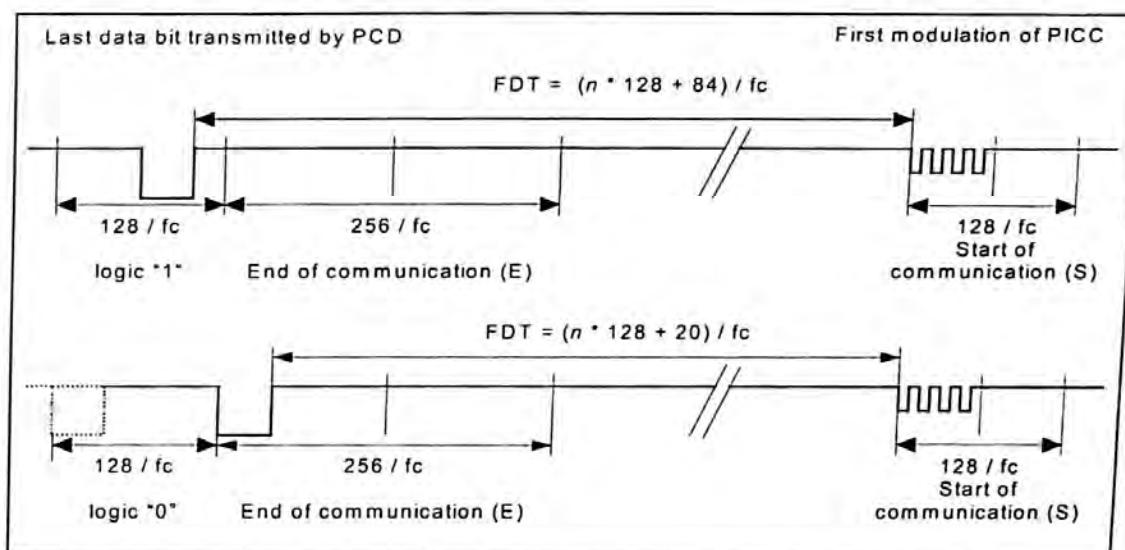
Figure 1 — Frame delay time PCD to PICC
