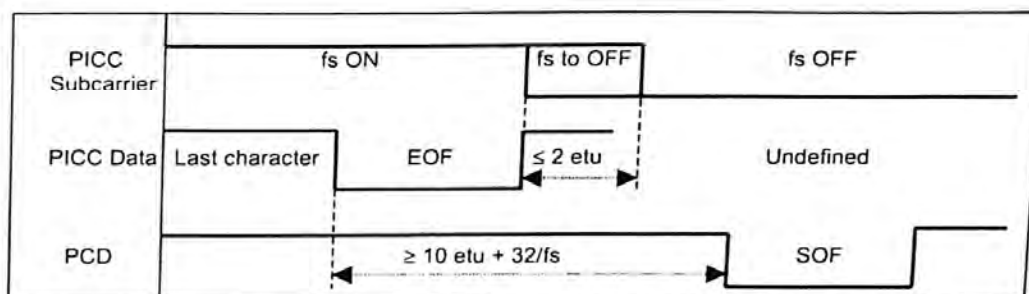
Figure 17 — PICC to PCD EOF
