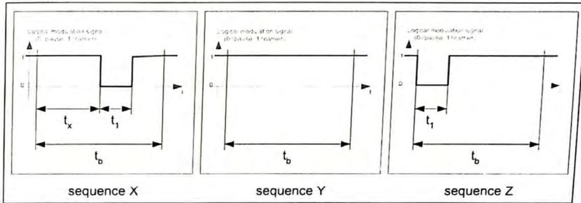
Figure Amd.1-3 — Signal shapes for sequences
