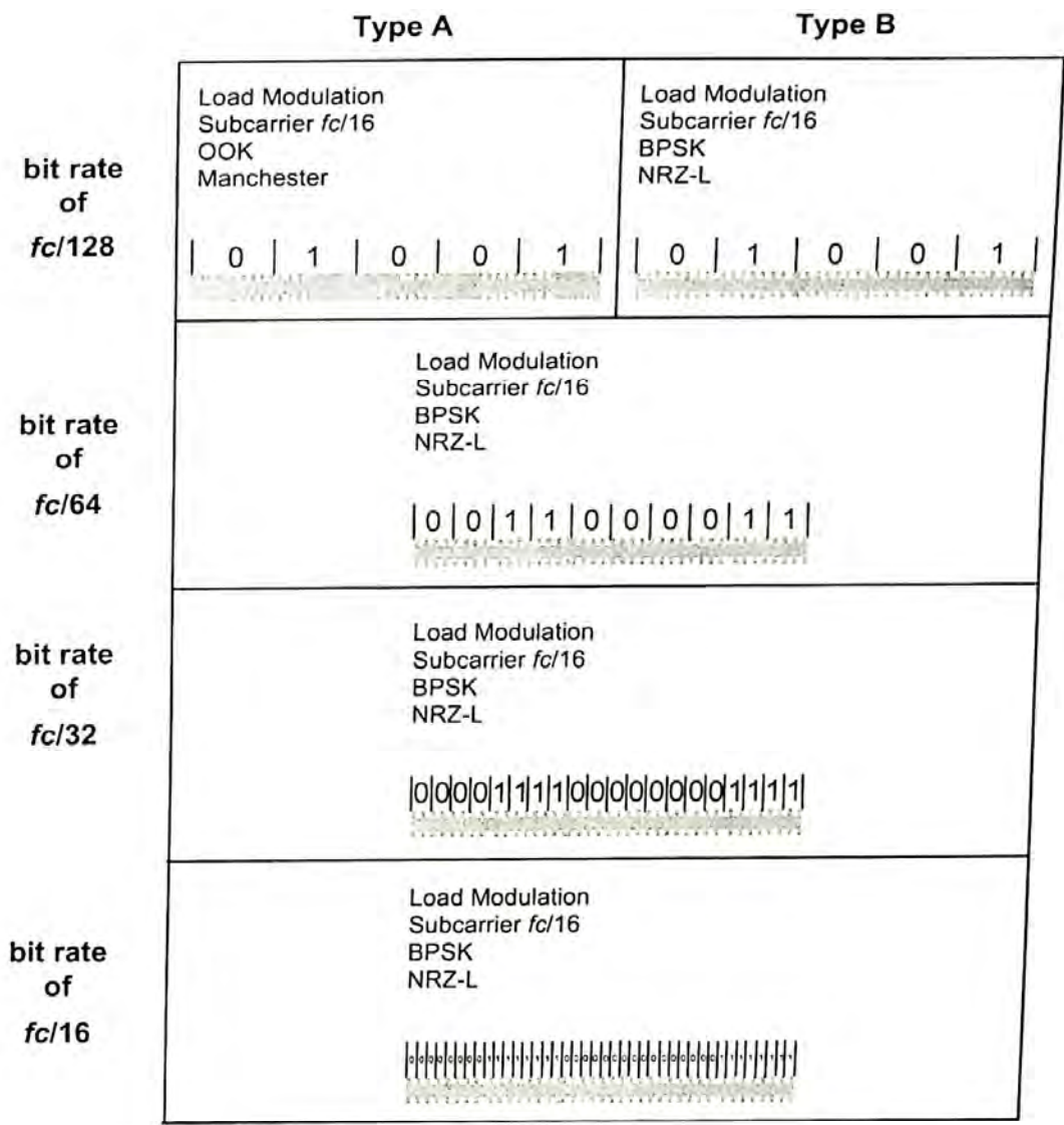
Figure Amd.1-1 — Example PICC to PCD communication signals for Type A and Type B interfaces
