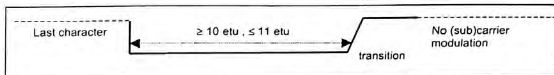
Figure 15 — EOF
