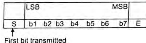
Figure 2 — Short frame
