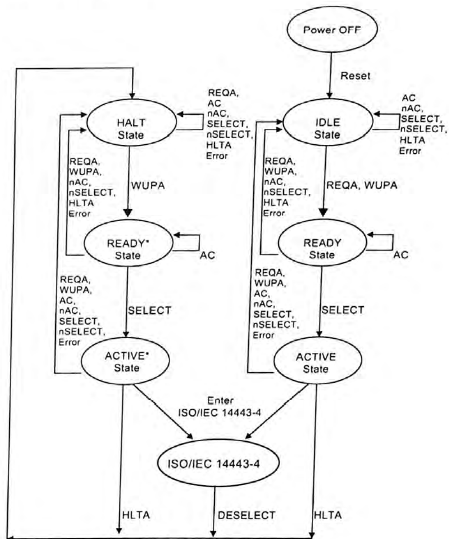
Figure 6 — PICC Type A state diagram
