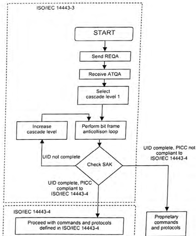
Figure 8 — Initialization and anticollision flowchart for PCD"
