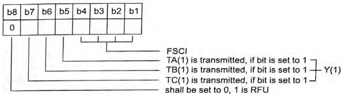
Figure 5 — Coding of format byte
