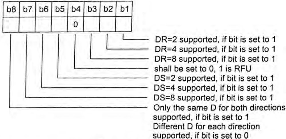
Figure 6 — Coding of interface byte TA(1)
