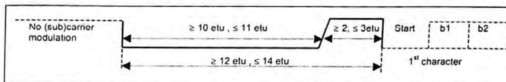
Figure 14 — SOF
