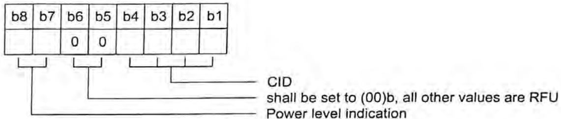
Figure 18 — Coding of card identifier
