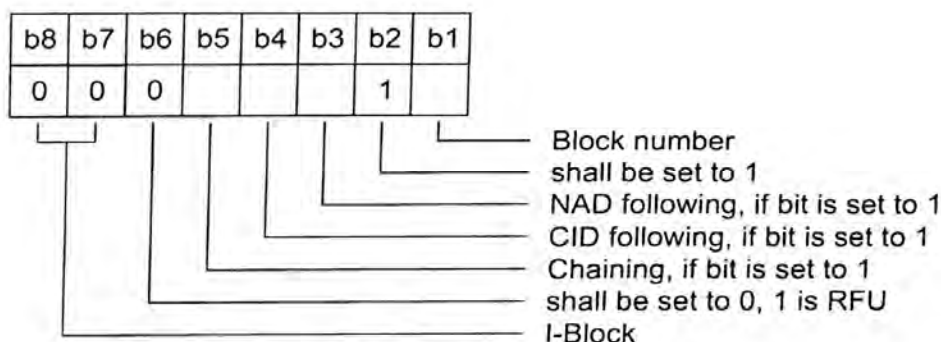
Figure 15 — Coding of I-block PCB
