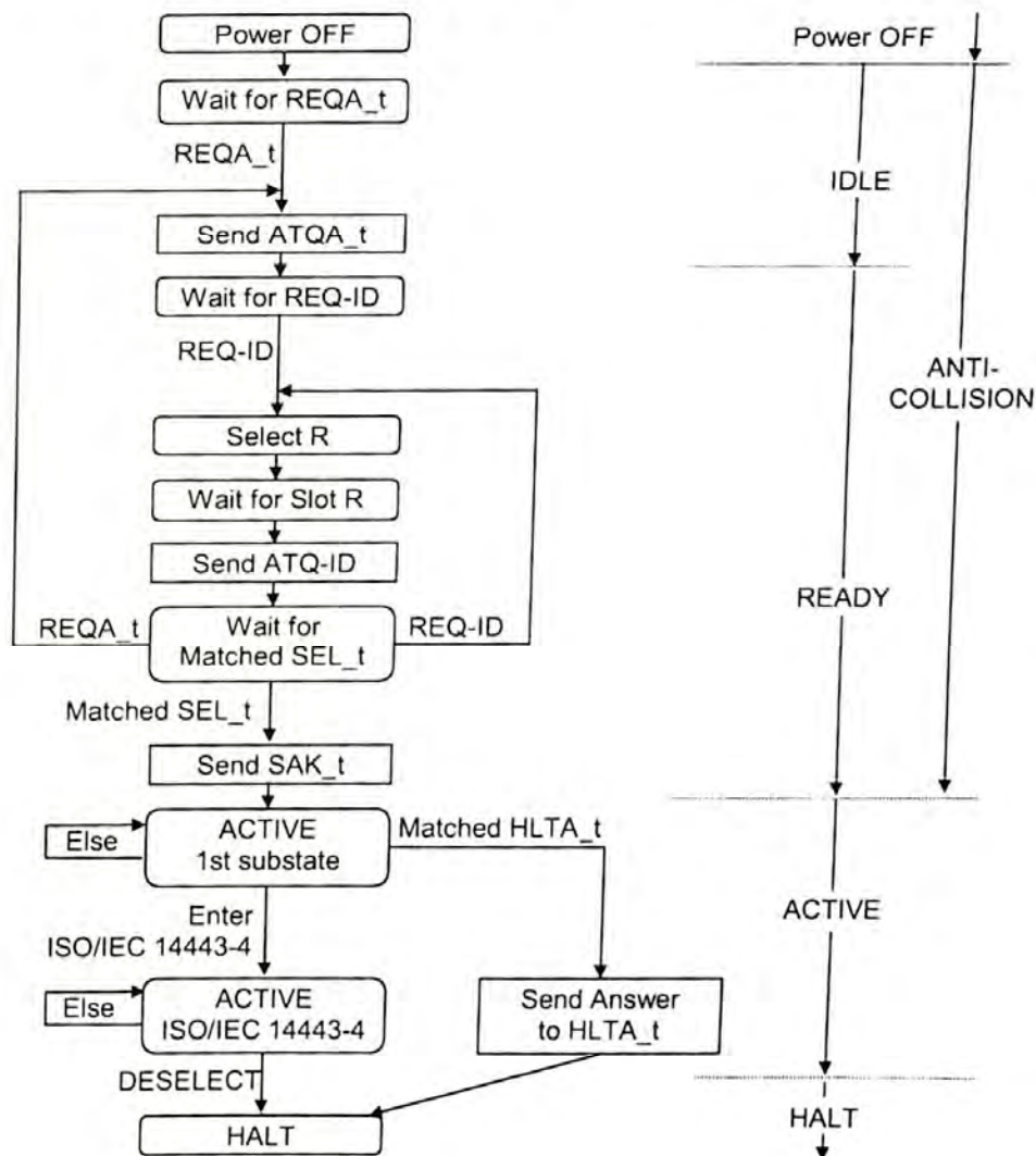
Figure C.1 — Flow chart of PICC anticollision sequence
