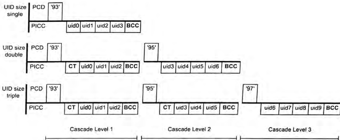
Figure 11 — Usage of cascade levels
