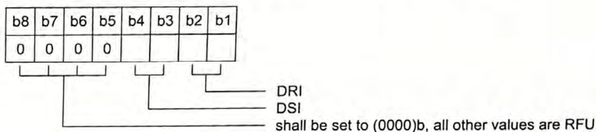
Figure 12 — Coding of PPS1
