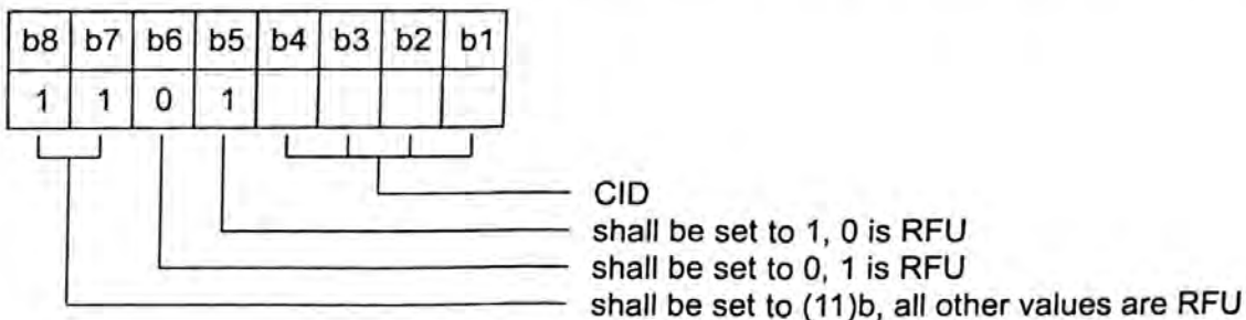
Figure 10 — Coding of PPSS
