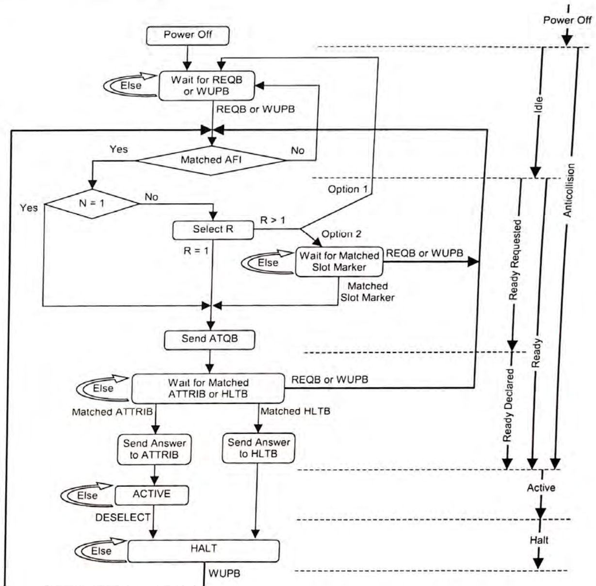
Figure 19 — PICC state transition flowchart example
