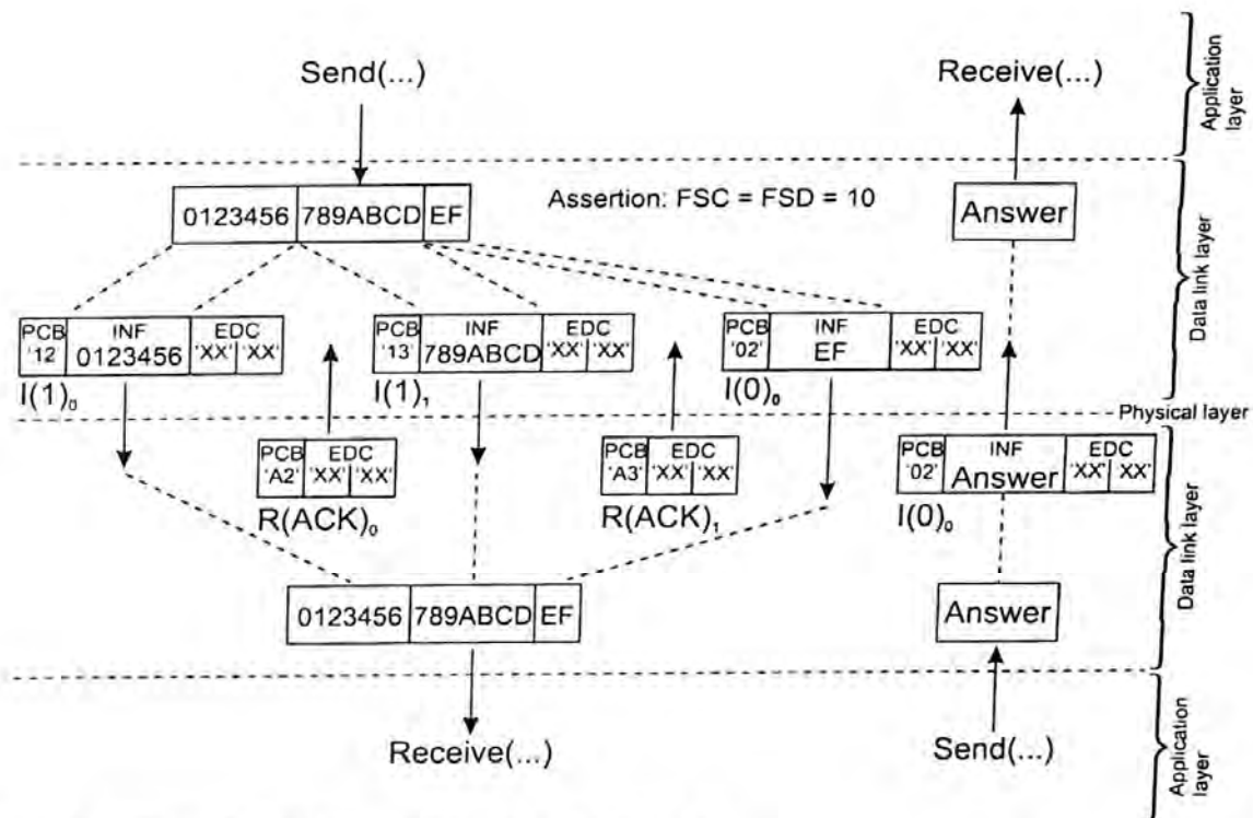
Figure 22 — Chaining
