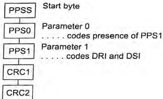
Figure 9 — Protocol and parameter selection request
