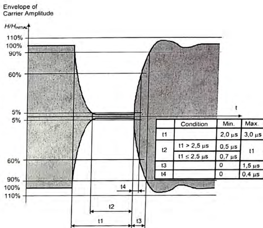
Figure 2 — Pause
