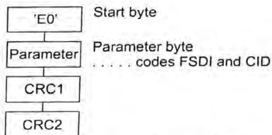
Figure 2 — Request for answer to select
