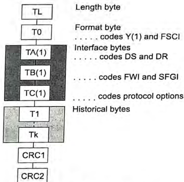
Figure 4 — Structure of the ATS
