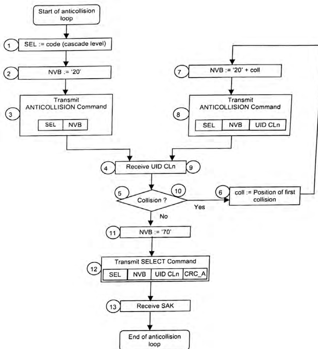
Figure 9 — Anticollision loop, flowchart for PCD
