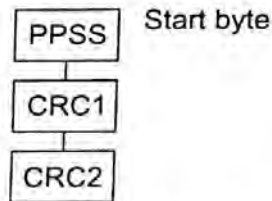
Figure 13 — Protocol and parameter selection response
