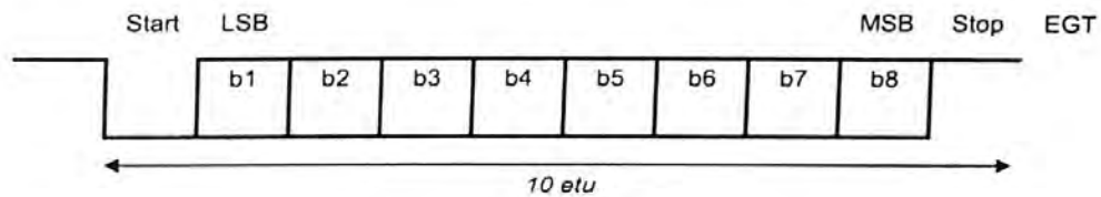
Figure 12 — Character format
