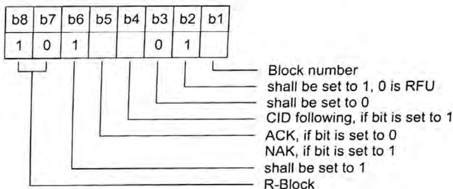
Figure 16 — Coding of R-block PCB
