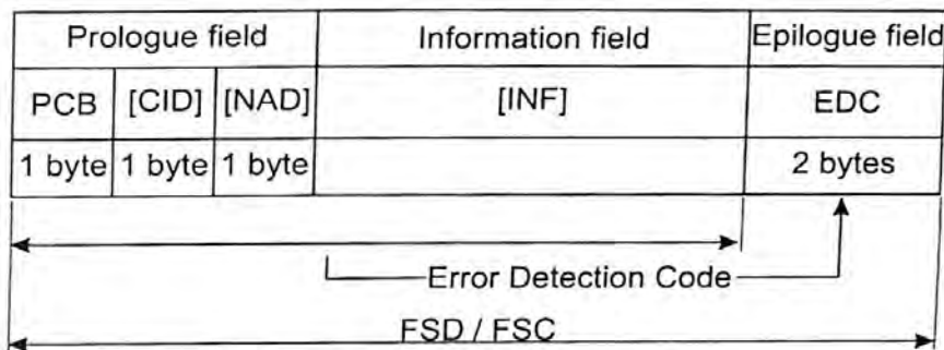
Figure 14 — Block format
