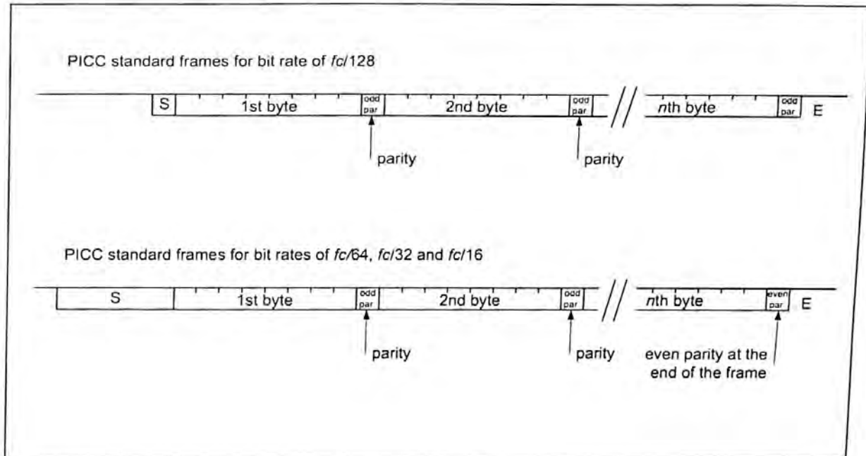
Figure Amd.1-1 — PICC standard frames"
