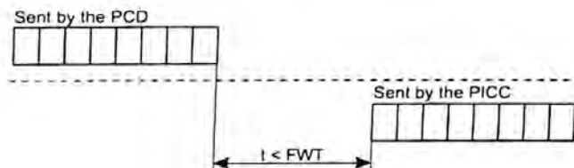
Figure 19 — Frame waiting time
