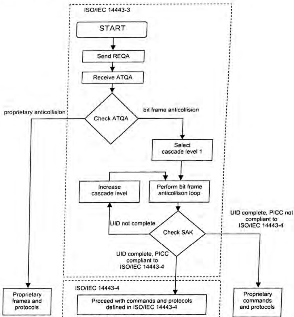
Figure 8 — Initialization and anticollision flowchart for PCD
