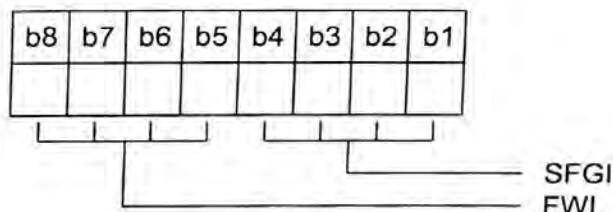
Figure 7 — Coding of interface byte TB(1)
