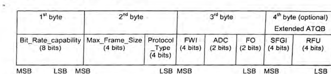
Figure 25 — Protocol Info format
