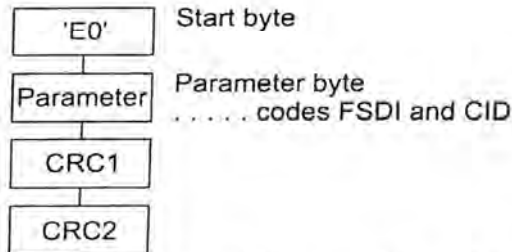
Figure 2 — Request for answer to select
