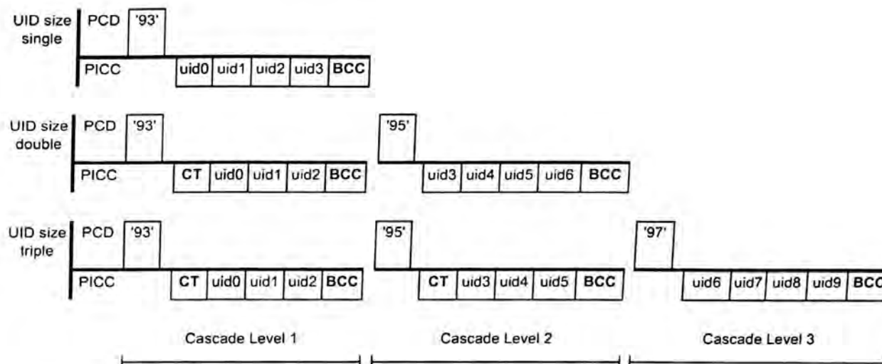
Figure 11 — Usage of cascade levels
