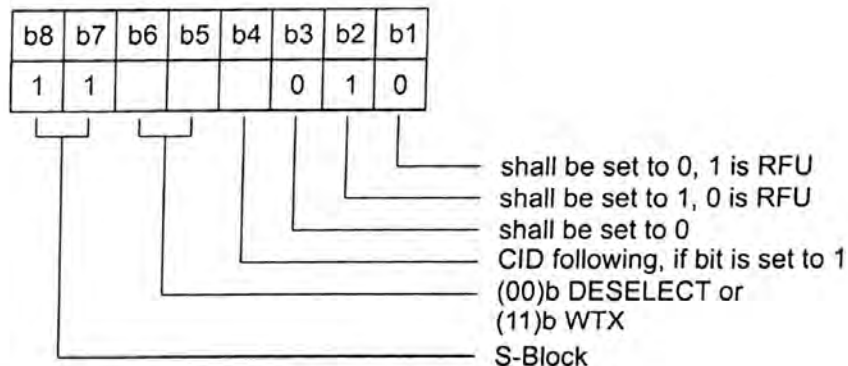
Figure 17 — Coding of S-block PCB
