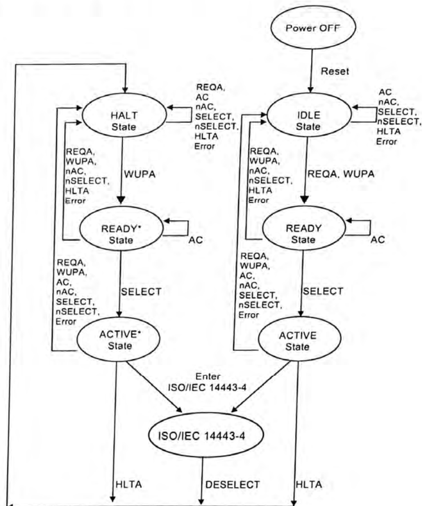
Figure 6 — PICC Type A state diagram
