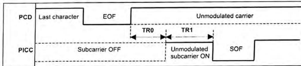
Figure 16 — PICC subcarrier SOF
