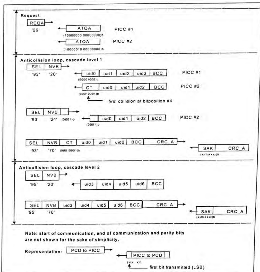
Figure A.1 — Select sequence with bit frame anticollision
