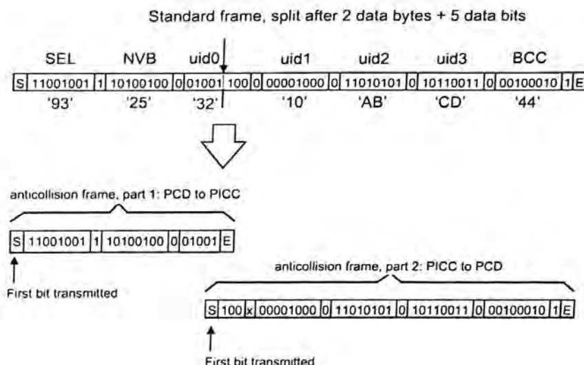
Figure 5 — Bit organization and transmission of bit oriented anticollision frame, case SPLIT BYTE
