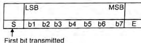
Figure 2 — Short frame
