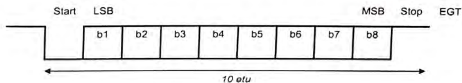
Figure 12 — Character format
