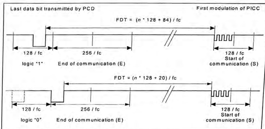
Figure 1 — Frame delay time PCD to PICC
