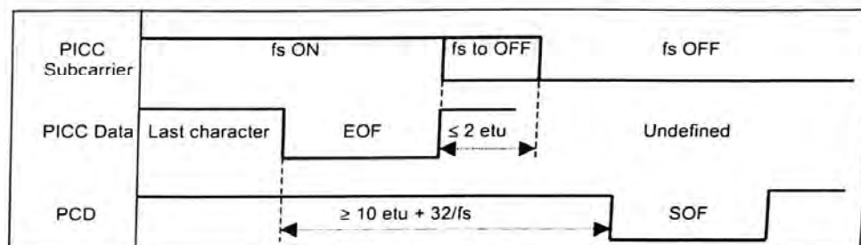
Figure 17 — PICC to PCD EOF
