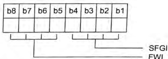
Figure 7 — Coding of interface byte TB(1)
