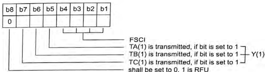
Figure 5 — Coding of format byte
