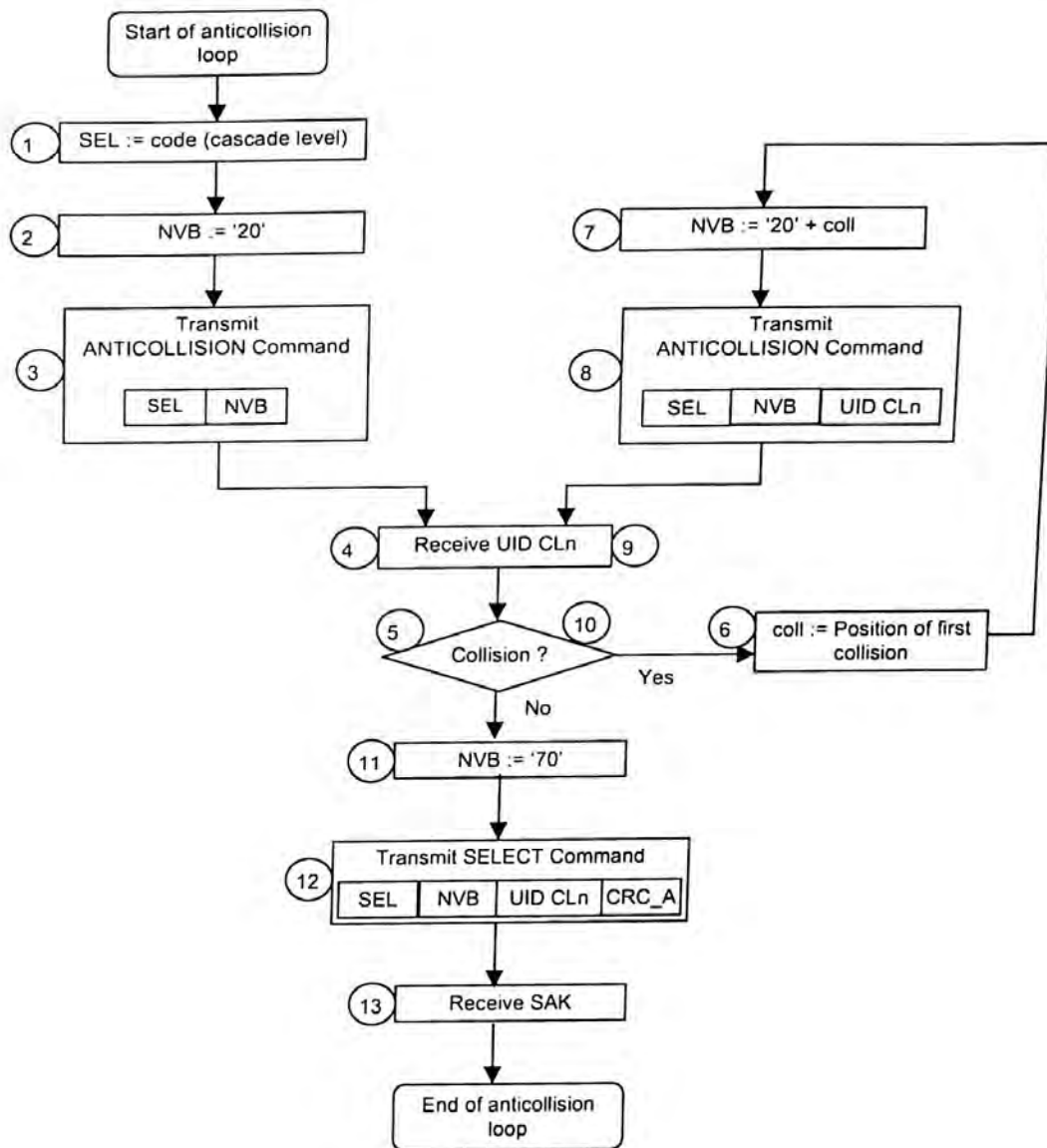
Figure 9 — Anticollision loop, flowchart for PCD
