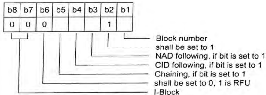
Figure 15 — Coding of I-block PCB
