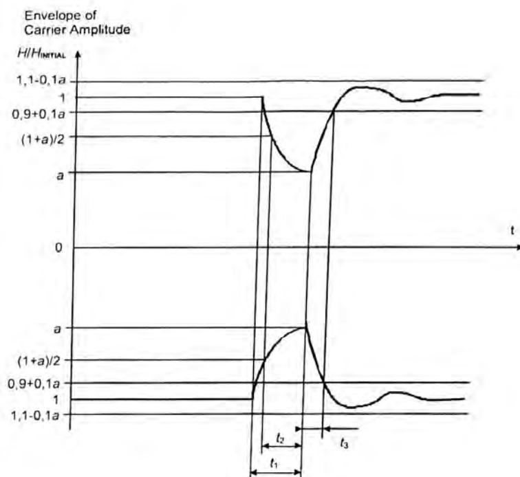
Figure Amd.1-2 — Pause for bit rates of fc/64 , fc/32 and fc/16
