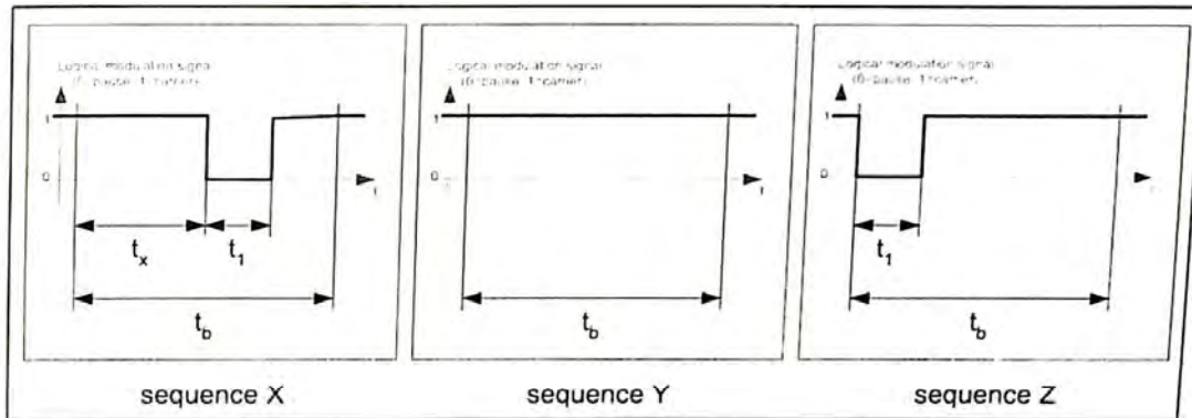
Figure Amd.1-3 — Signal shapes for sequences
