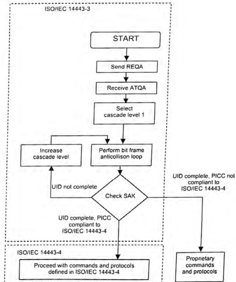
Figure 8 — Initialization and anticollision flowchart for PCD"
