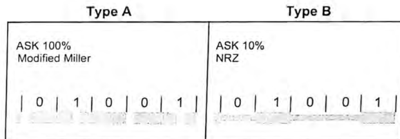
Figure 1 — Example PCD to PICC communication signals for Type A and Type B interfaces
