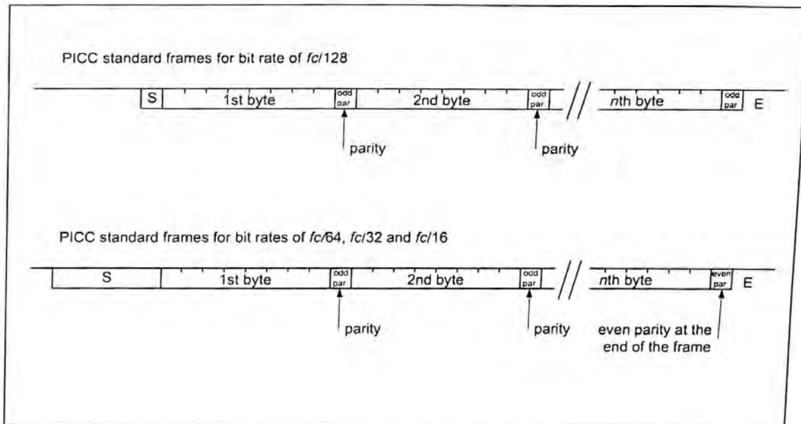
Figure Amd.1-1 — PICC standard frames"
