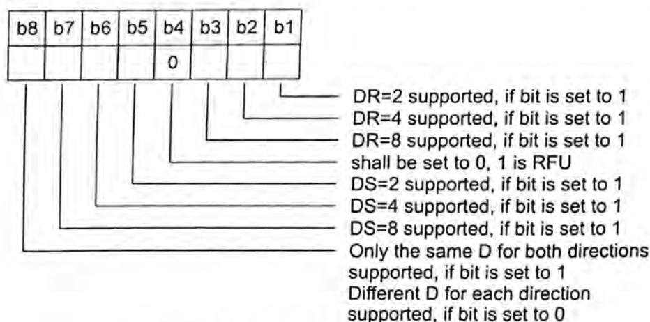
Figure 6 — Coding of interface byte TA(1)
