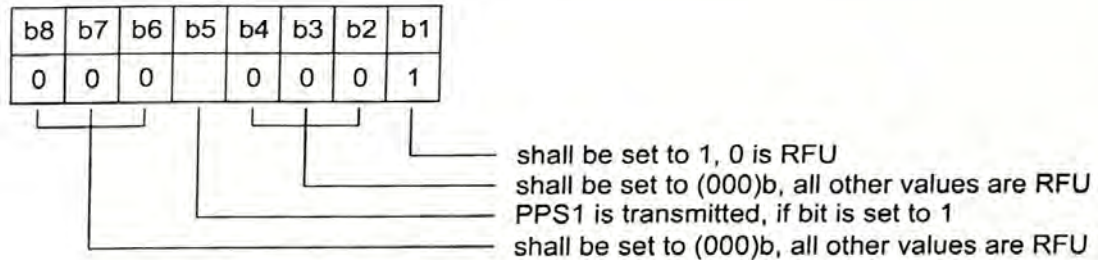
Figure 11 — Coding of PPS0
