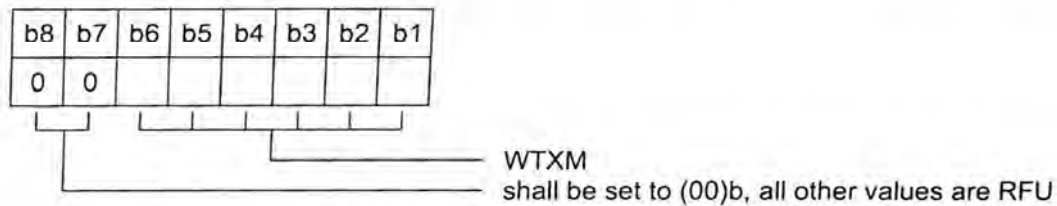
Figure 21 — Coding of INF field of an S(WTX) response
