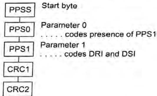
Figure 9 — Protocol and parameter selection request
