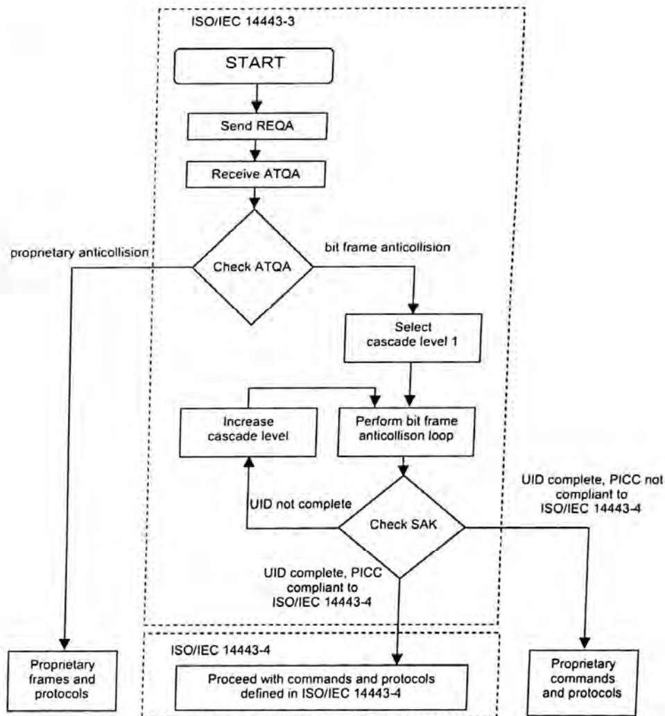
Figure 8 — Initialization and anticollision flowchart for PCD
