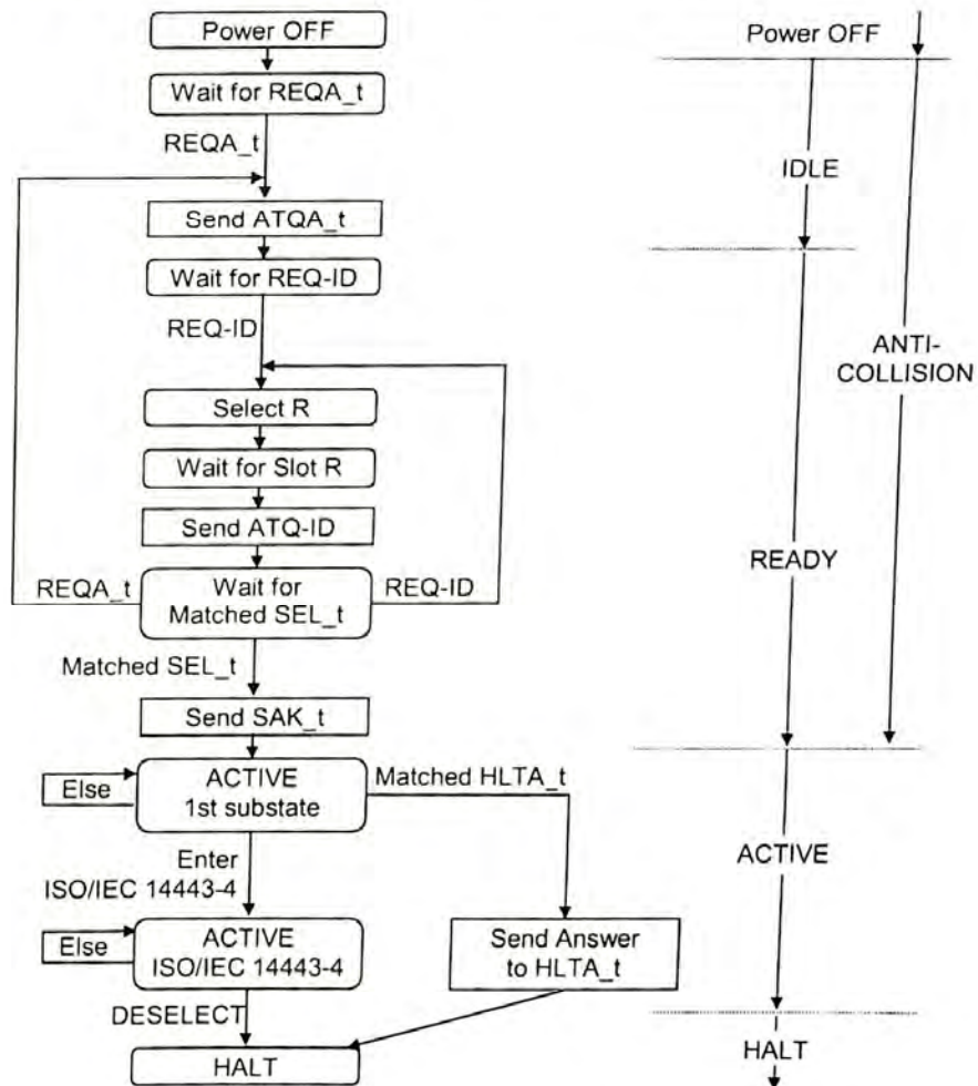
Figure C.1 — Flow chart of PICC anticollision sequence
