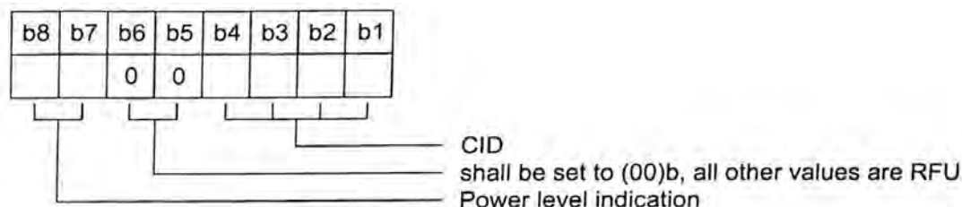
Figure 18 — Coding of card identifier
