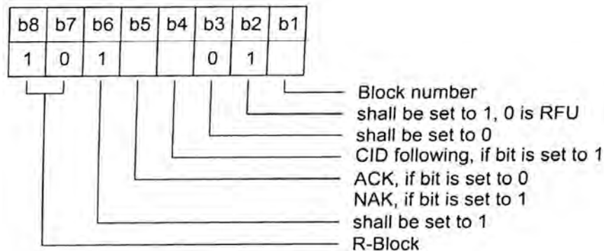
Figure 16 — Coding of R-block PCB
