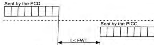
Figure 19 — Frame waiting time
