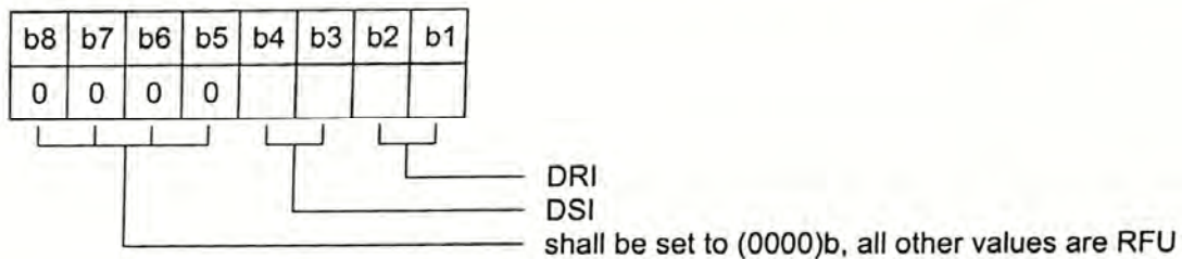
Figure 12 — Coding of PPS1
