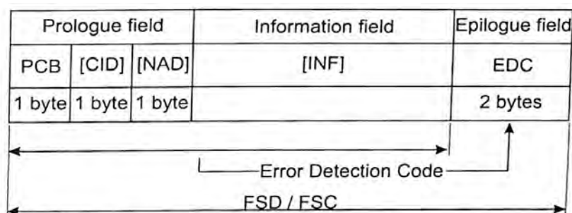
Figure 14 — Block format
