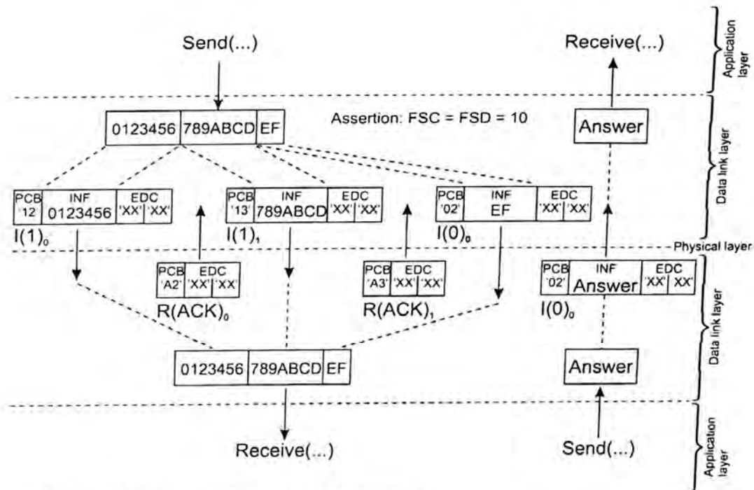
Figure 22 — Chaining
