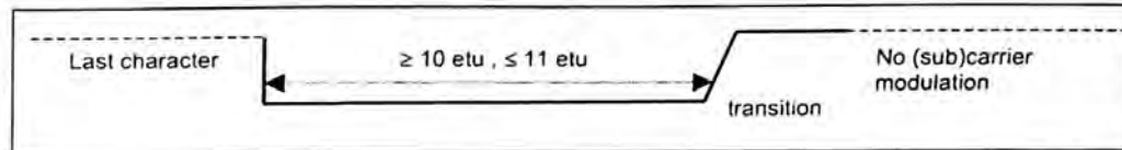
Figure 15 — EOF
