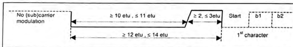
Figure 14 — SOF
