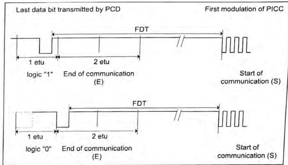
Figure 1 — Frame delay time PCD to PICC"
