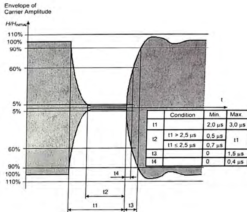
Figure 2 — Pause
