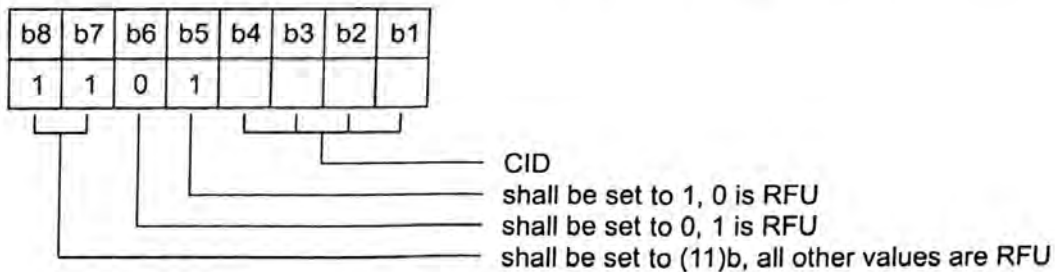
Figure 10 — Coding of PPSS
