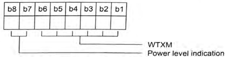
Figure 20 — Coding of INF field of an S(WTX) request
