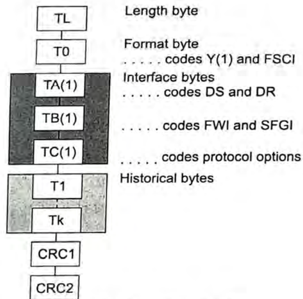
Figure 4 — Structure of the ATS
