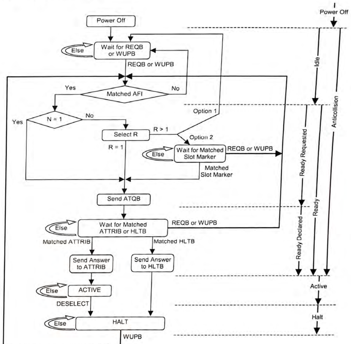
Figure 19 — PICC state transition flowchart example
