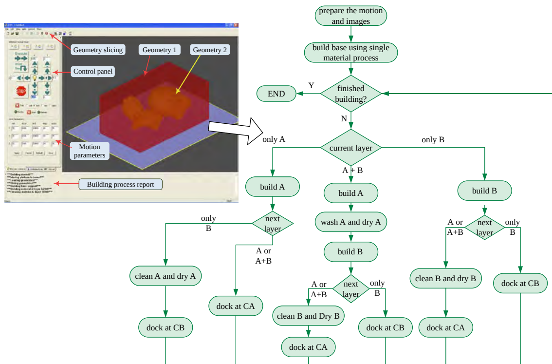
Figure 12 Flow chart of the multi-materials MIP-SL system and related software system
