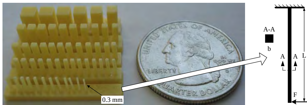
Figure 9 Shearing force verification test
