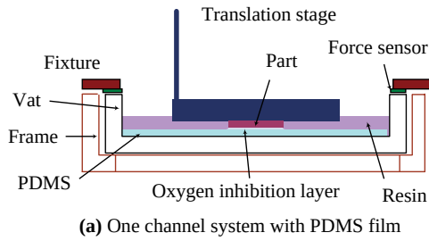
Figure 4 Experimental setup for studying part separation forces in the MIP-SL process
