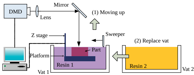
Figure 2 An illustration of the multi-material SL process based on top-down projection
