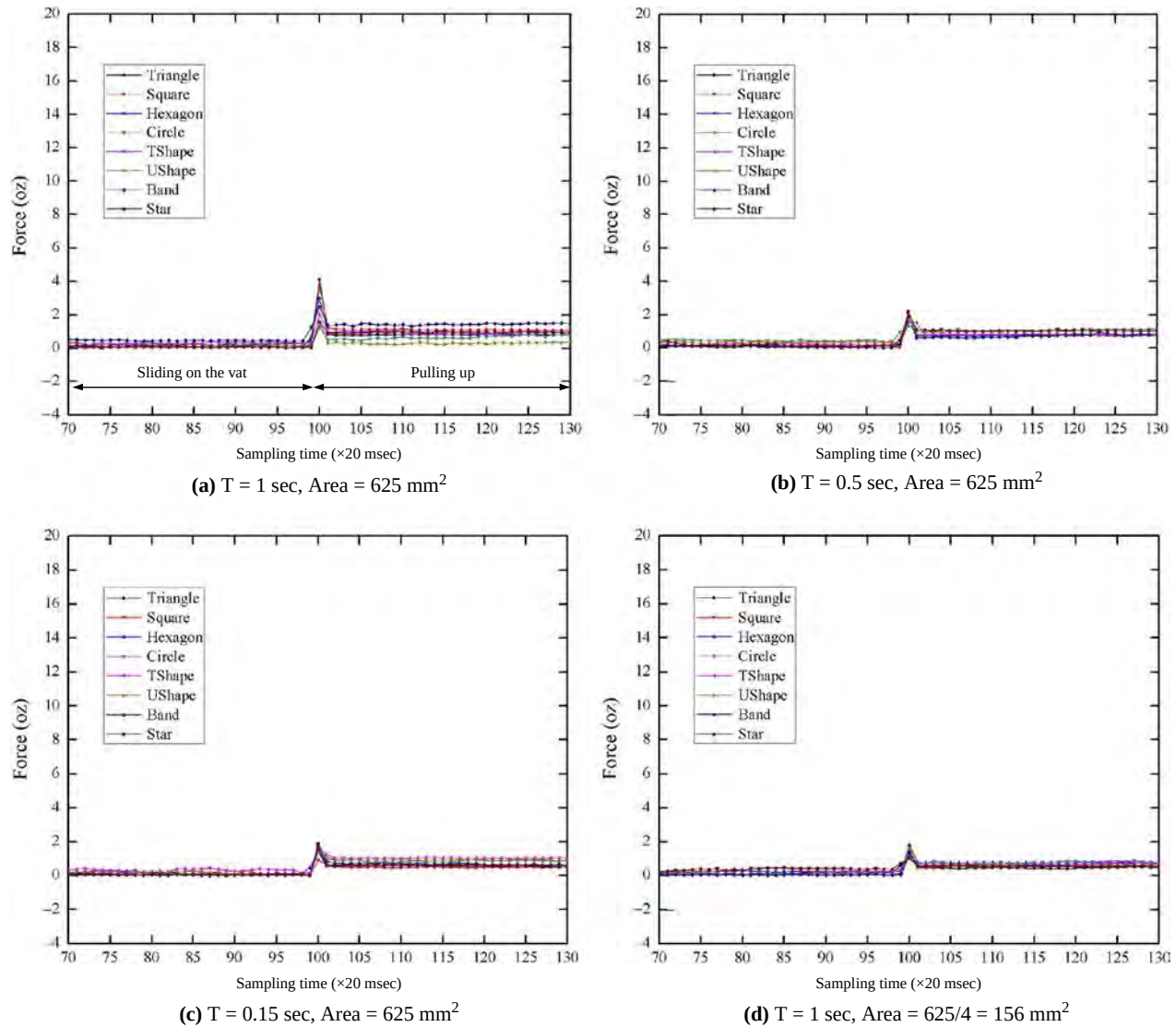
Figure 8 Pulling forces of cured layer for two-channel system in different test cases
