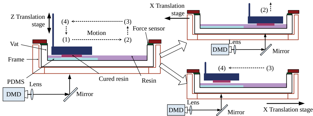
Figure 7 Two-channel system with PDMS
