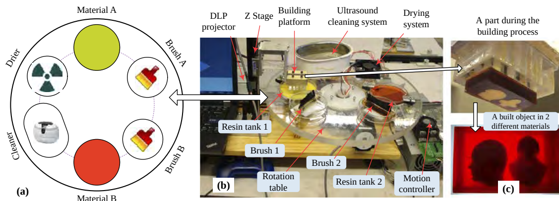
Figure 11 Hardware system of the prototype multi-material MIP-SL system
