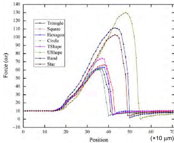
Figure 5 Pulling forces of cured layer from a PDMS film in different test cases
