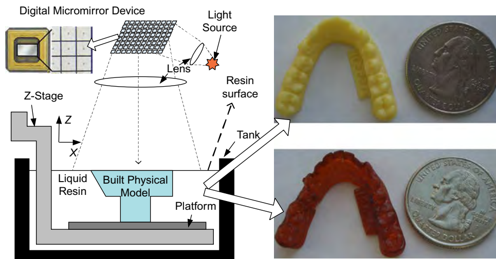
Figure 1 An illustration of the MIP-SL process
