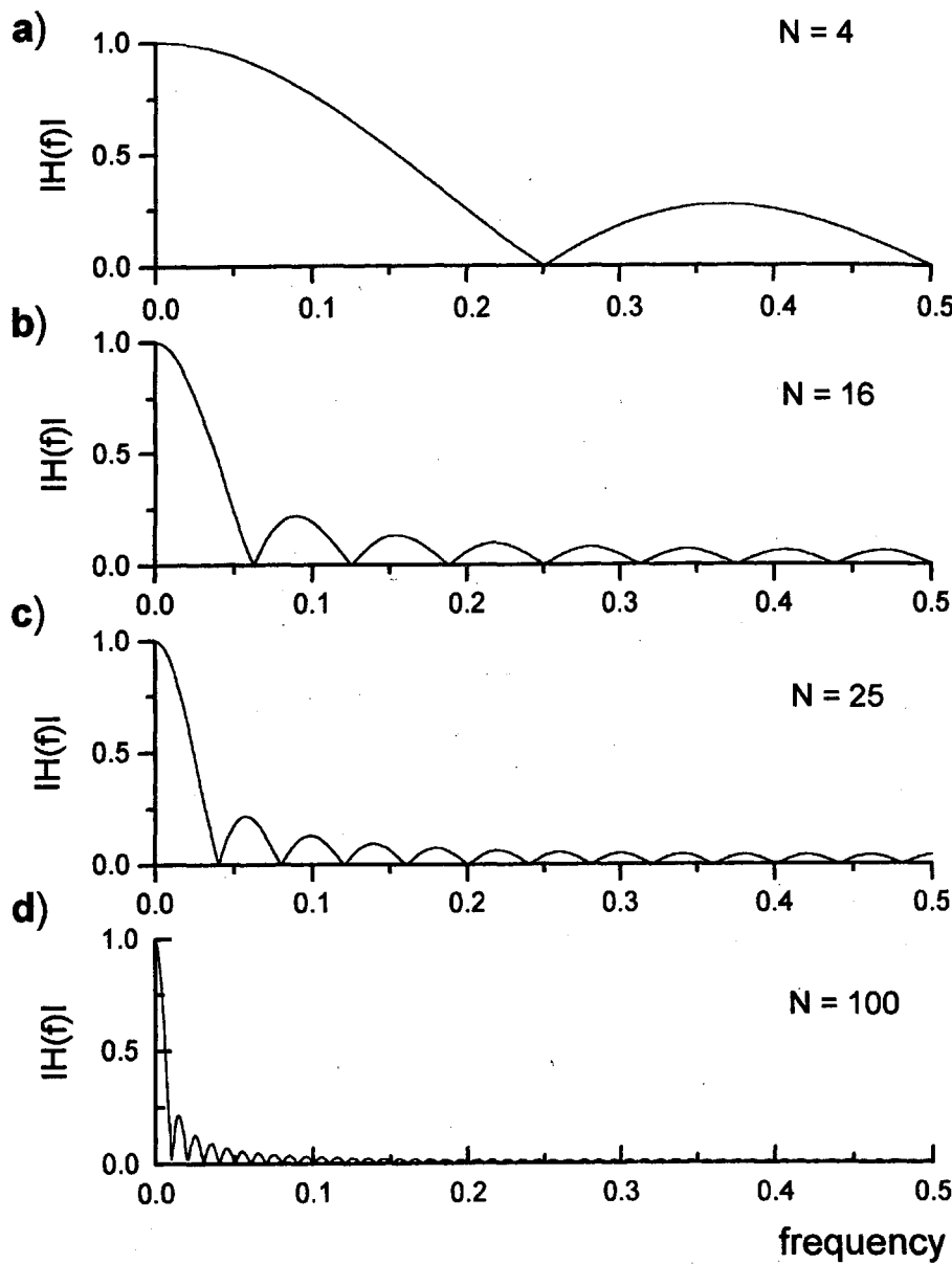
FIGURE 55.14 Equivalent frequency response for the signal-averaging procedure for different values of N (see text).
