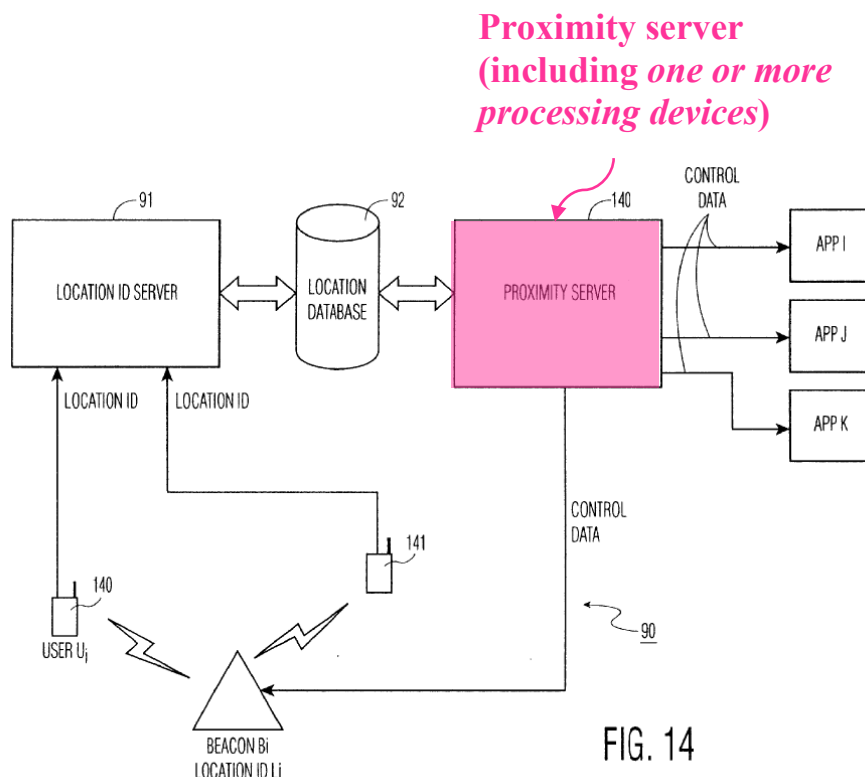
Rachabathuni, FIG. 14 (annotated)
