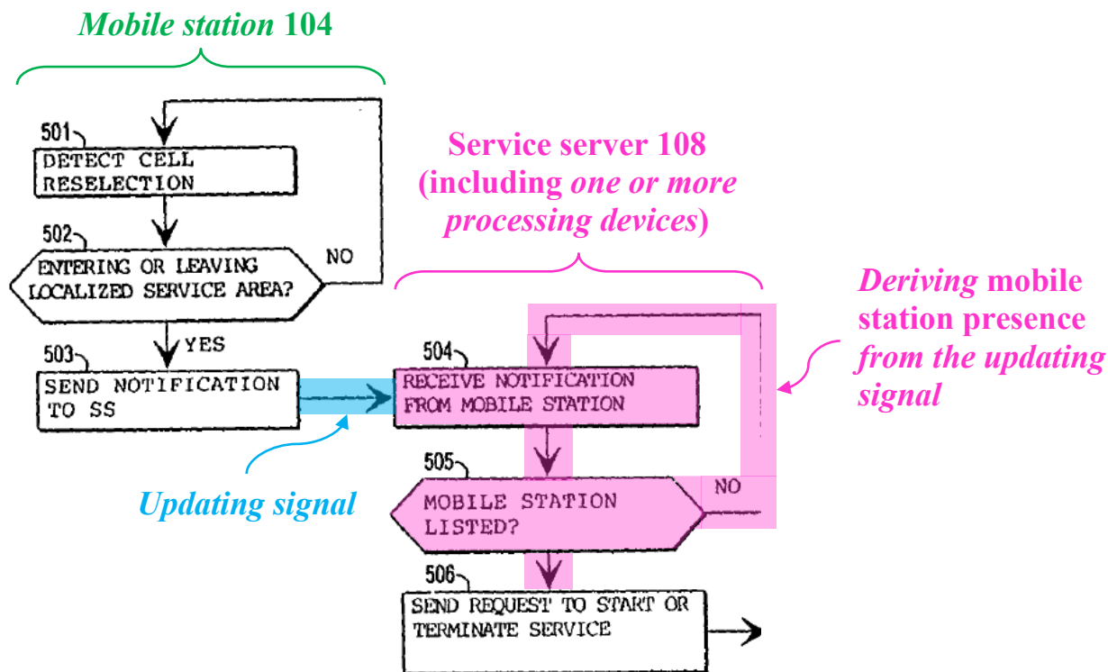
Putkiranta, Detail of FIG. 5 (annotated)
