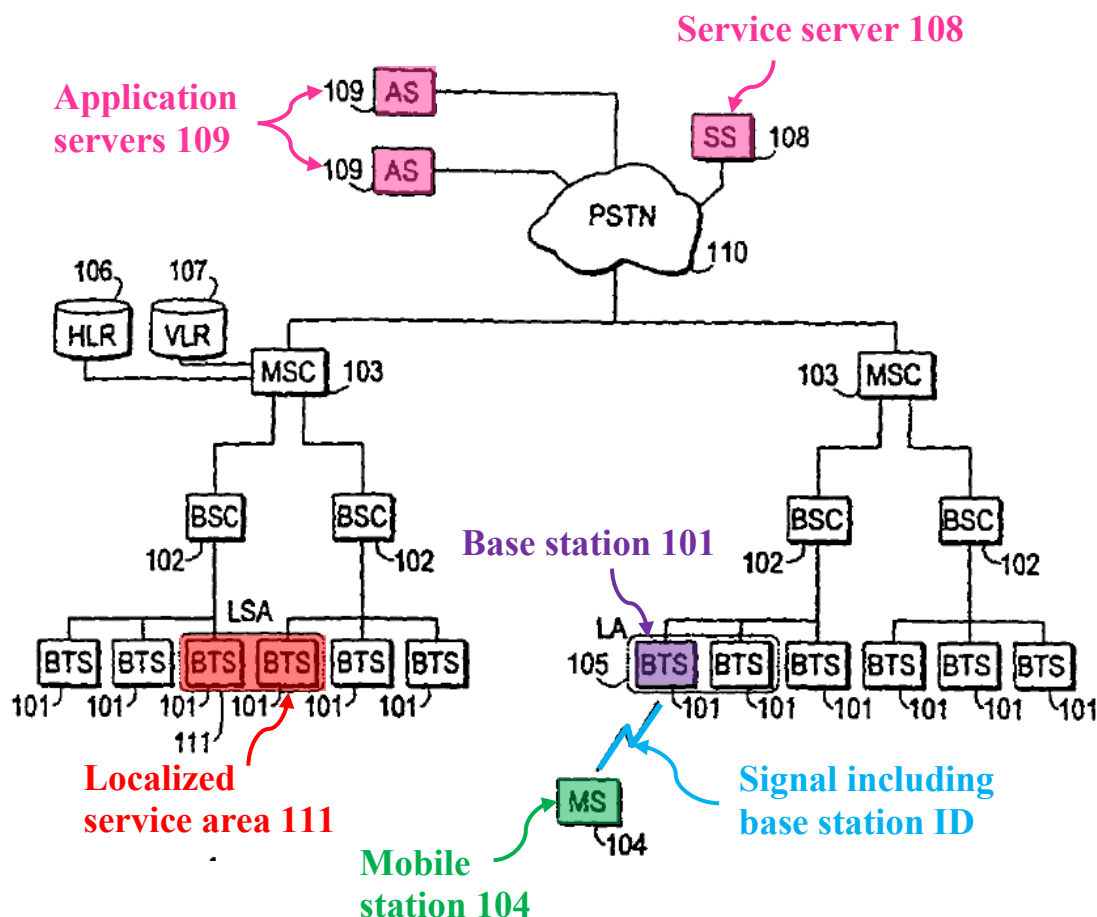
Putkiranta, Detail of FIG. 1 (annotated)
