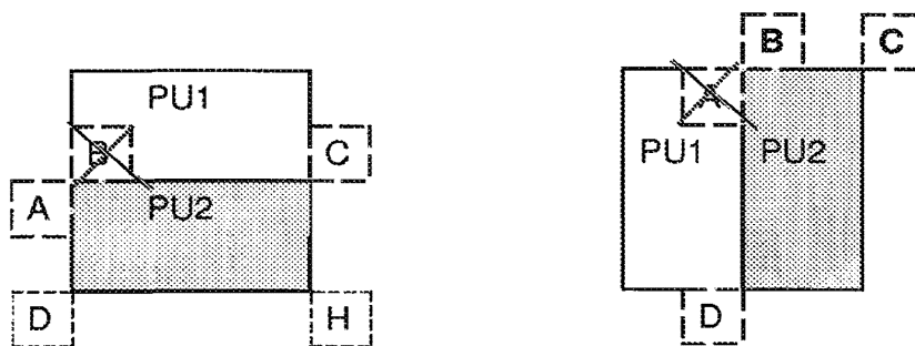
Figure 7. An example of removing redundant MVPs in 2NxN and Nx2N Merge mode to avoid imitation.
