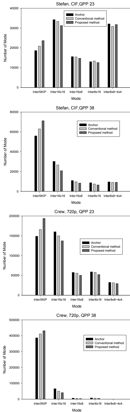
Fig. 3. Mode used for each block mode in sequence
