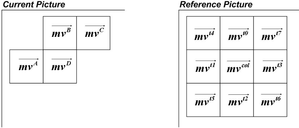
Fig. 1. Motion vector of current block(D) and spatially neighboring blocks(A, B, and C) in current picture, and temporally co-located block(Col) and others(t0~t7) in reference picture.
