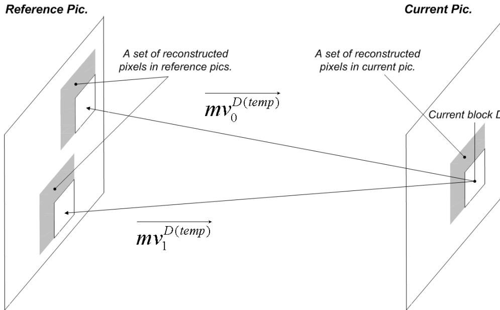
Fig. 2. Optimal PMV Estimation at Decoder using Template Matching
