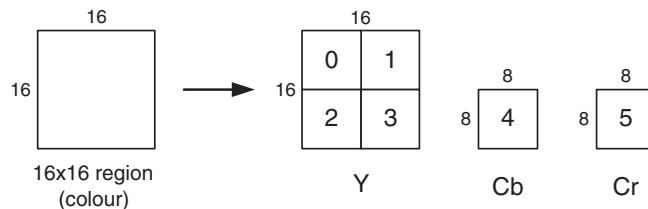
Figure 3.8 Macroblock (4:2:0)
