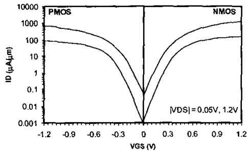
Fig. 7: NMOS and PMOS subthreshold curves.
