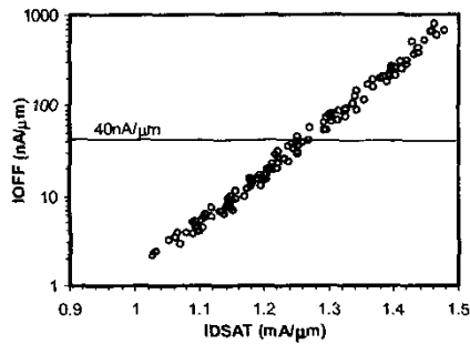
Fig. 11: NMOS I_{DSAT} vs. I_{OFF} at 1.2V
