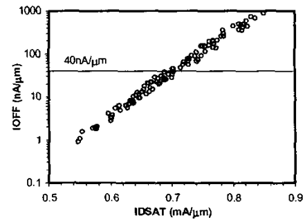
Fig. 10: PMOS I_{DSAT} vs. I_{OFF} at 1.2V
