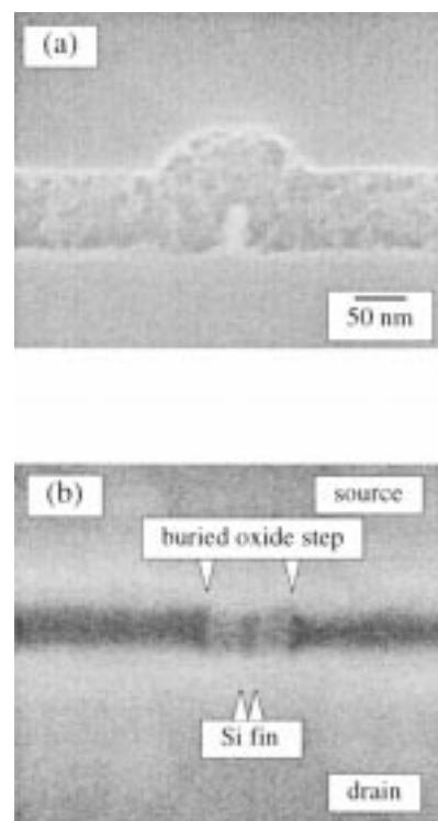
Fig. 3. (a) Cross-sectional SEM picture of 15-nm Si vertical fin. The height is 50 nm. (b) Top view of channel region after spacer etching. The spacer gap between source and drain is 50 nm.
