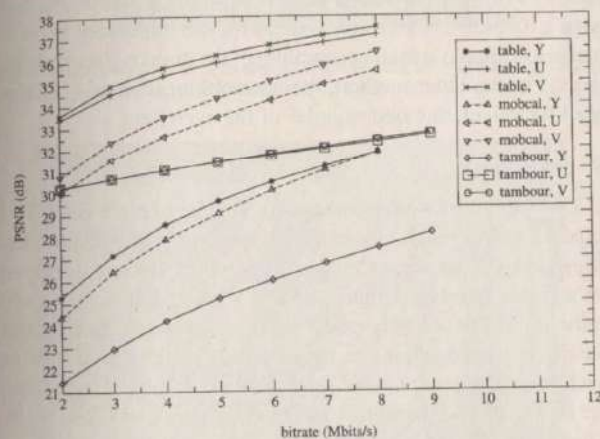
Fig. 5. PSNR of directly decoded sequences as a function of the bit rate.
