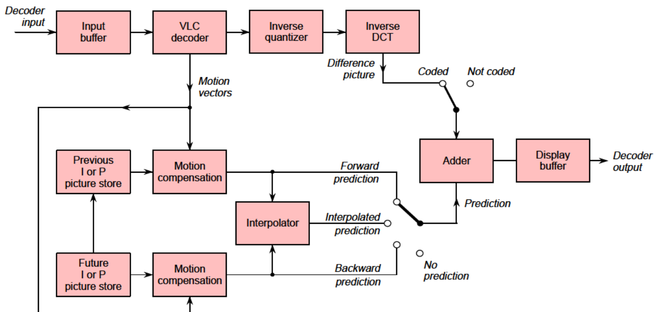
Figure 12 Decoding a "B" macroblock.
