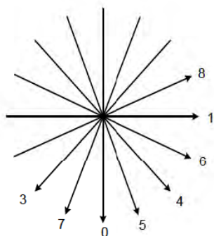
Figure 8-1 – Intra_4x4 prediction mode directions (informative)
