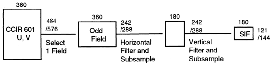
(b) Chrominance
