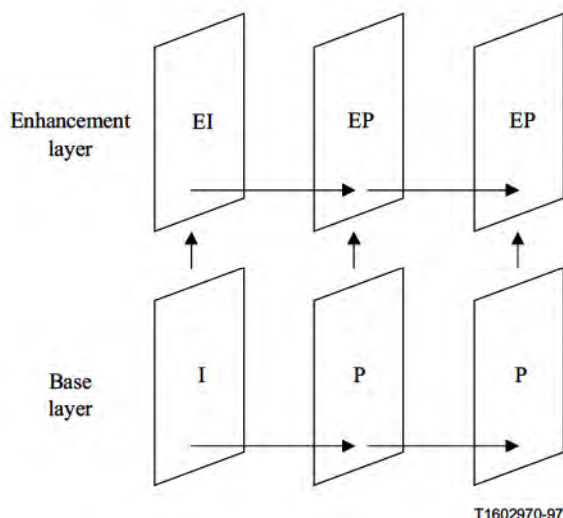
Figure O.2/H.263 – Illustration of SNR scalability
