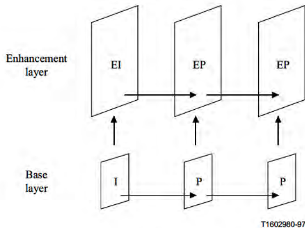
Figure O.3/H.263 – Illustration of spatial scalability
