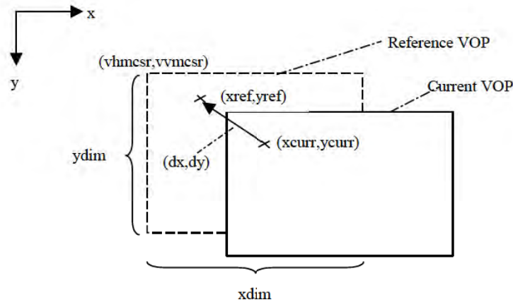
Figure 7-33 — Unrestricted motion compensation
