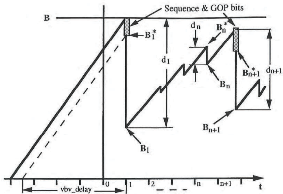
Figure C.1 -- VBV buffer occupancy
