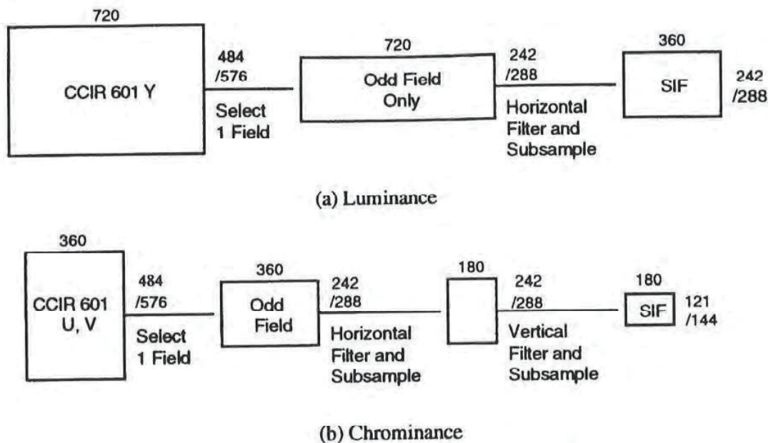
Figure D.12 -- Conversion from CCIR 601 into SIF
