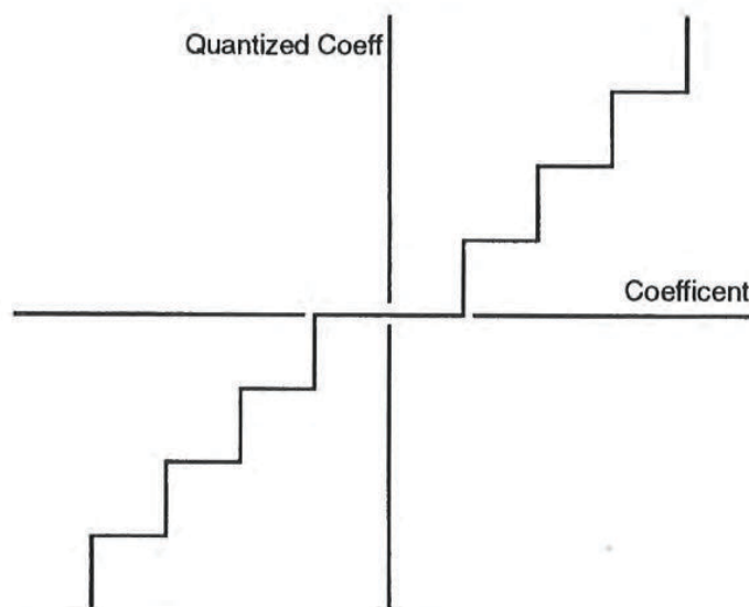
Figure D.35 -- Dead zone quantizer characteristic
