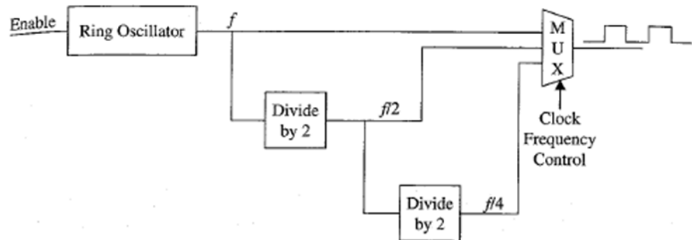
Figure 5-3 Variable frequency clock generator.
