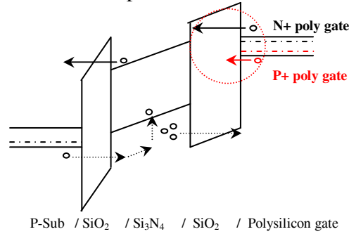
Figure 3. Energy band diagram of n + polysilicon and p + polysilicon gate SONOS when negative voltage is applied to the gate in erasure process.
