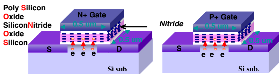
Figure 1. Schematics of n^+ type and p^+ type polysilicon gate SONOS.
