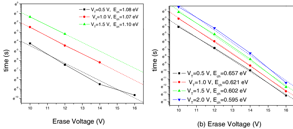
Figure 8. Emission characteristic energy of (a) n^+ polysilicon gate and (b) p^+ polysilicon gate SONOS.
