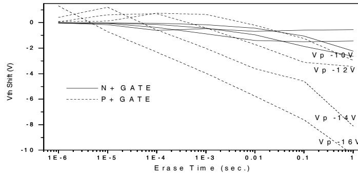
Figure 7. Erasing speed characteristics of n^+ and p^+ gate.
