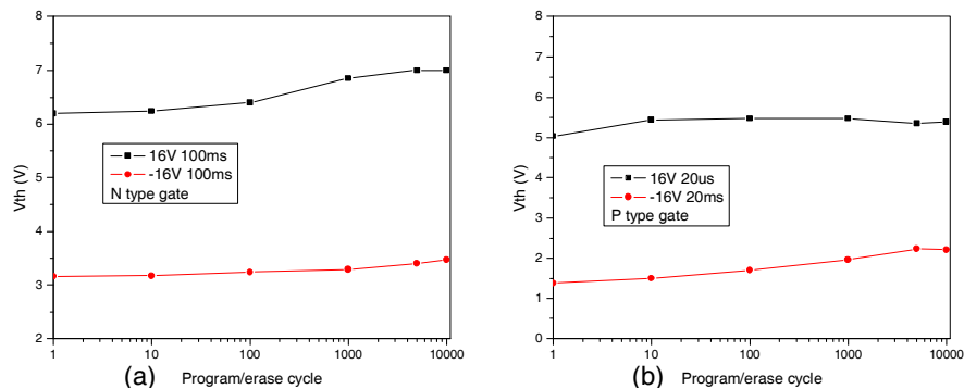
Figure 9. Endurance characteristics of (a) n^+ and (b) p^+ polysilicon gate memories.
