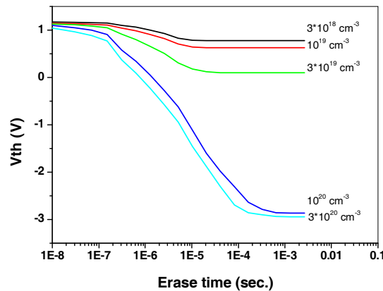
Figure 4. Threshold voltage dependence on boron doping concentrations of polysilicon gates in erasure mode.
