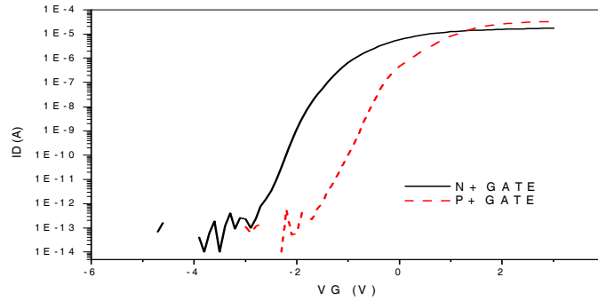
Figure 5. Transfer characteristics of n^+ and p^+ polysilicon gates at 0.5V drain voltage.
