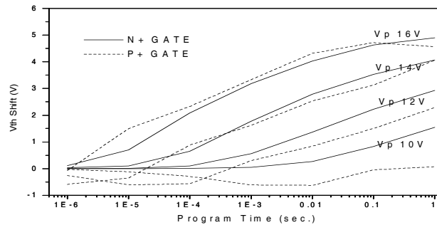
Figure 6. Programming speed characteristics of n^+ and p^+ gate.
