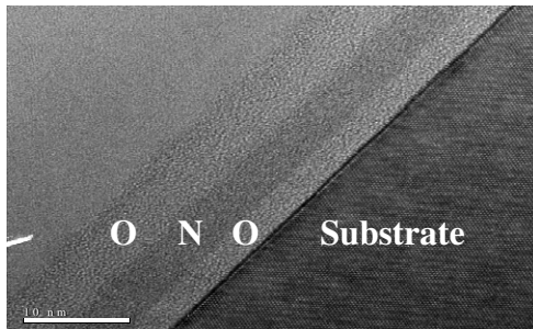
Figure 2. Transmission-electron-micrograph (TEM) of the ONO stack (3 nm / 5.5 nm / 7 nm).
