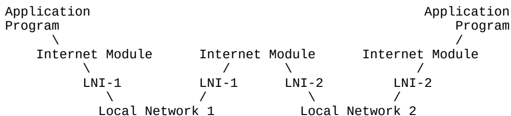
Transmission Path
