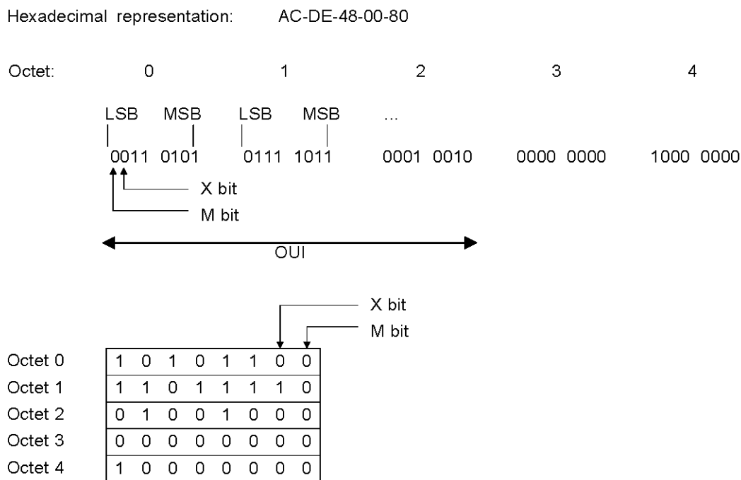
Figure 9—Protocol identifier
