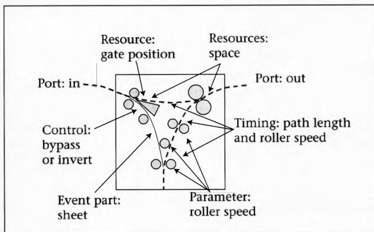
Figure 4. Constraints Are Derived from Physical Model of the Inverter.
