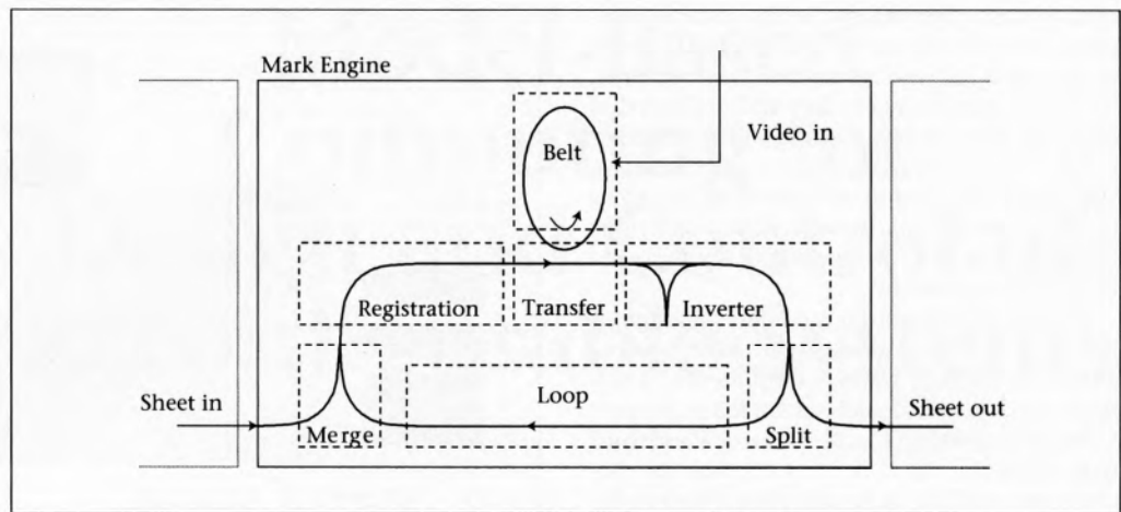
Figure 2. Schematic Decomposition of a Machine's Paper Path.
