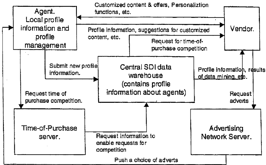
Figure 17, Time-of-Purchase/Amazon-like system
