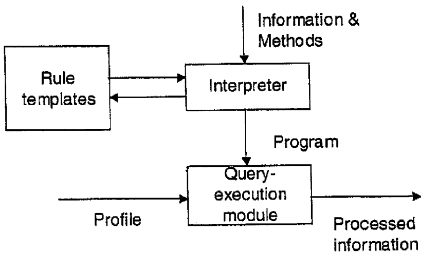
Figure 7. Client-side Personalization.
