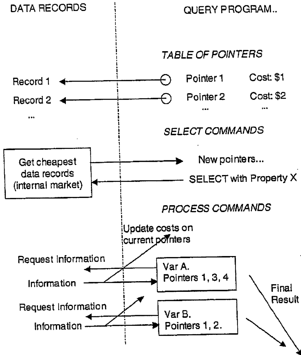
Figure 3: Query Execution
