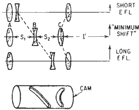
Figure 9.31 Mechanically compensated zoom system.
