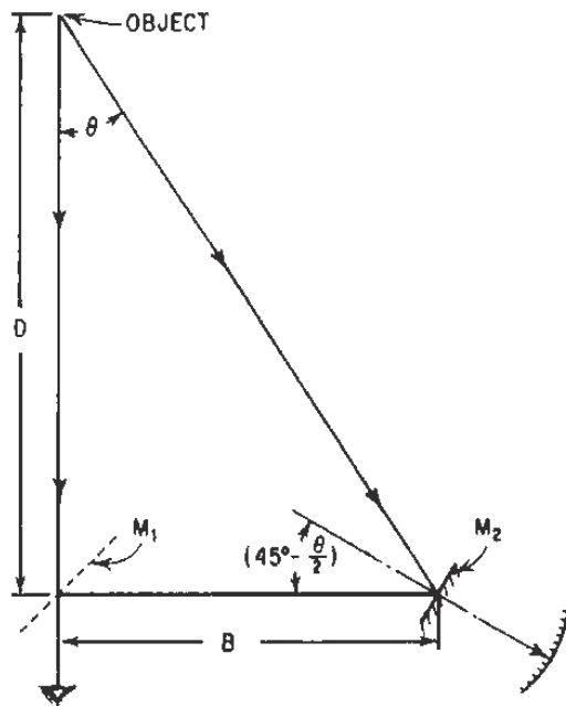
Figure 9.13 Basic rangefinder optical system. The eye views the object directly through semi-reflector M_1 and also through movable mirror M_2 . The angular setting of M_2 which brings both views into coincidence determines the range.
