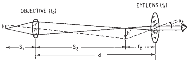
Figure 9.12 The compound microscope.
