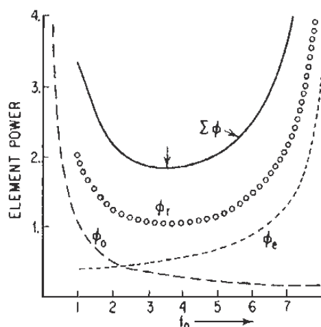
Figure 9.9 Plot of the element powers for a 10-in-long erecting telescope with 4-in eye relief versus the arbitrarily chosen objective focal length. \phi_o , \phi_r , and \phi_e are the powers of the objective, erector, and eyelens, respectively.
