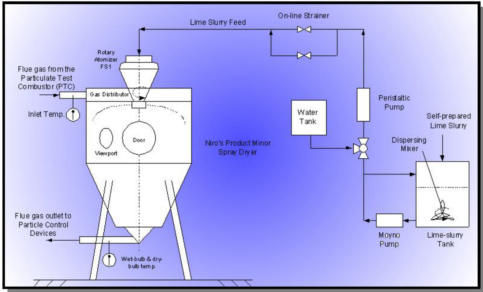
Spray Dryer Flow Diagram
