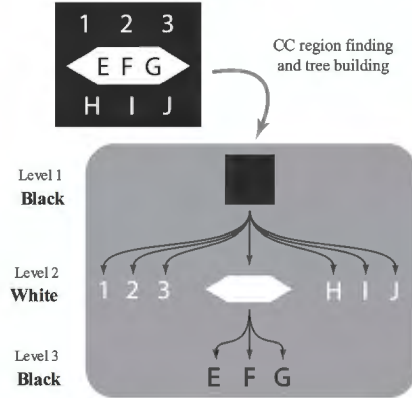
Figure 1. A synthetic sample image and its corresponding tree of connected regions.
