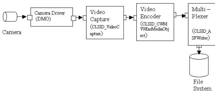
Figure 1: Filter Graph for Video Capture
