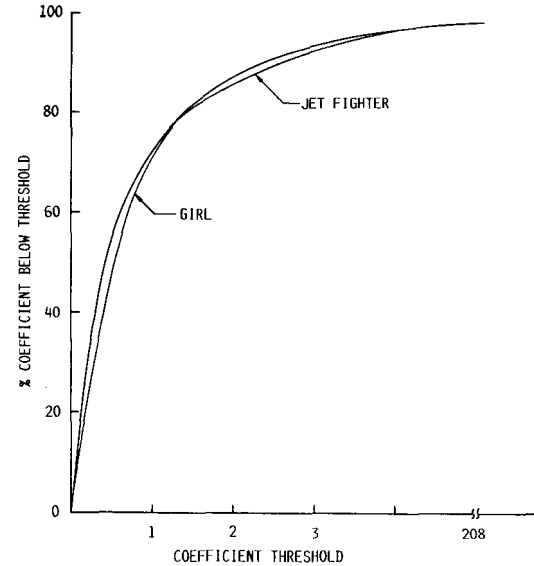
Fig. 3. Distribution of cosine transform coefficients.
