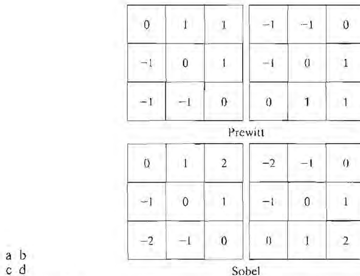
FIGURE 10.9 Prewitt and Sobel masks for detecting diagonal edges.
