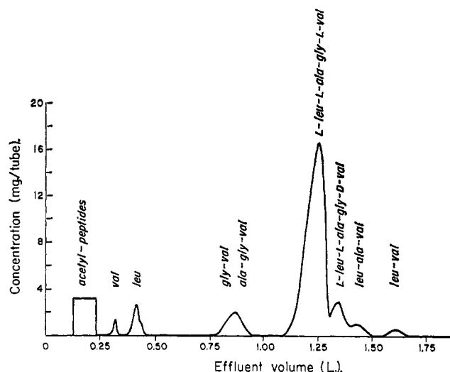
Fig. 2.—Chromatographic separation of the tetrapeptide L-leucyl-L-alanylglycyl-L-valine on a 2 × 120 cm. column of Dowex 50-X4 resin. Elution was with 0.1 M pyridine acetate buffer, pH 4.0. The concentration was calculated from the ninhydrin analysis of individual tubes and dry weight of pooled fractions.
