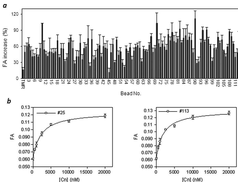
Figure 2. Evaluation of the binding affinity of the 113 hits to Cn by fluorescence anisotropy. (a) Comparison of all 113 hits at a fixed concentration of Cn (5 \mu M) and TMR-labeled cyclic peptide (100 nM). The percentage of FA increase was relative to the anisotropy value of the corresponding peptide in the absence of Cn. (b) Plots of FA values as a function of the Cn concentration for cyclic peptides derived from beads No. 25 and 113. The curves were fitted to the data as described under Experimental Procedures. All measurements were performed in triplicate.
