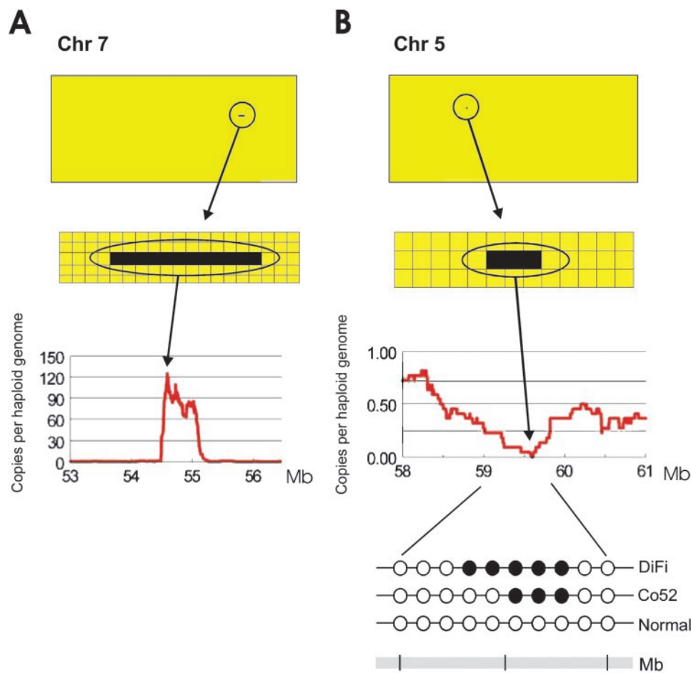
Fig. 3. High-resolution tag density maps identify amplifications and deletions. (A) Amplification on chromosome 7. (Top) A bitmap viewer with the region containing the alteration encircled. The bitmap viewer is comprised of \approx 39,000 pixels representing tag density values at the chromosomal position of each virtual tag on chromosome 7, determined from sliding windows of 50 virtual tags. Yellow pixels indicate tag densities corresponding to copy numbers of <110 , while black pixels correspond to copy numbers \geq 110 . (Middle) An enlarged view of the region of alteration. (Bottom) A graphical representation of the amplified region with values on the y axis indicating genome copies per haploid genome and values on the x axis representing positions along the chromosome in Mb. (B) Homozygous deletion on chromosome 5. Top, Middle, and Bottom are similar to those for A except that the bitmap viewer for chromosome 5 contains \approx 43,000 pixels, tag density values were calculated in sliding windows of 150 virtual tags, and yellow pixels indicate copy numbers >0.1 while black pixels indicate copy numbers \leq 0.1 . (Bottom) Below the graph is a detailed analysis of the region containing the homozygous deletion in DiFi and Co52. For each sample, white dots indicate markers that were retained, while black dots indicate markers that were homozygously deleted. PCR primers for each marker are listed in Table 4.
